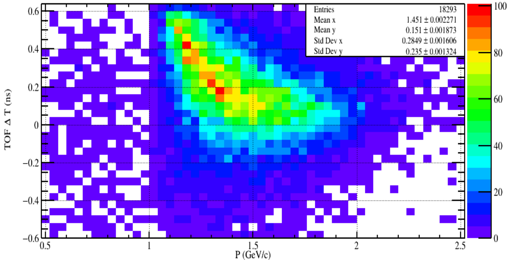
\Delta T Vs P: Proton Timing in TOF (MC)
