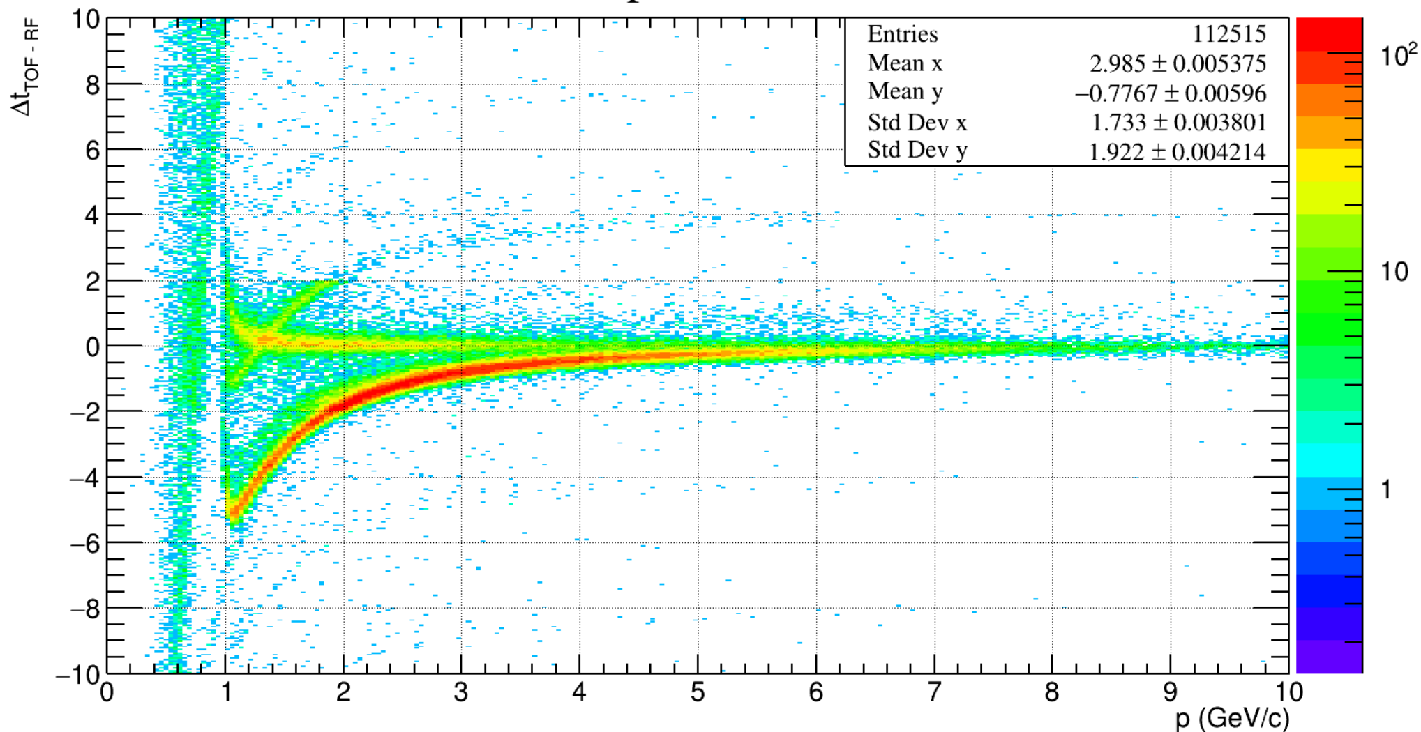
TOF p Candidates
