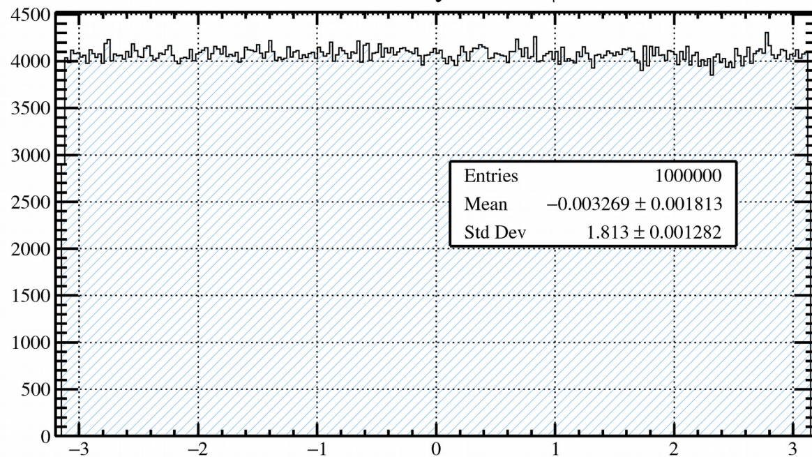
K + Helicity Frame \phi
