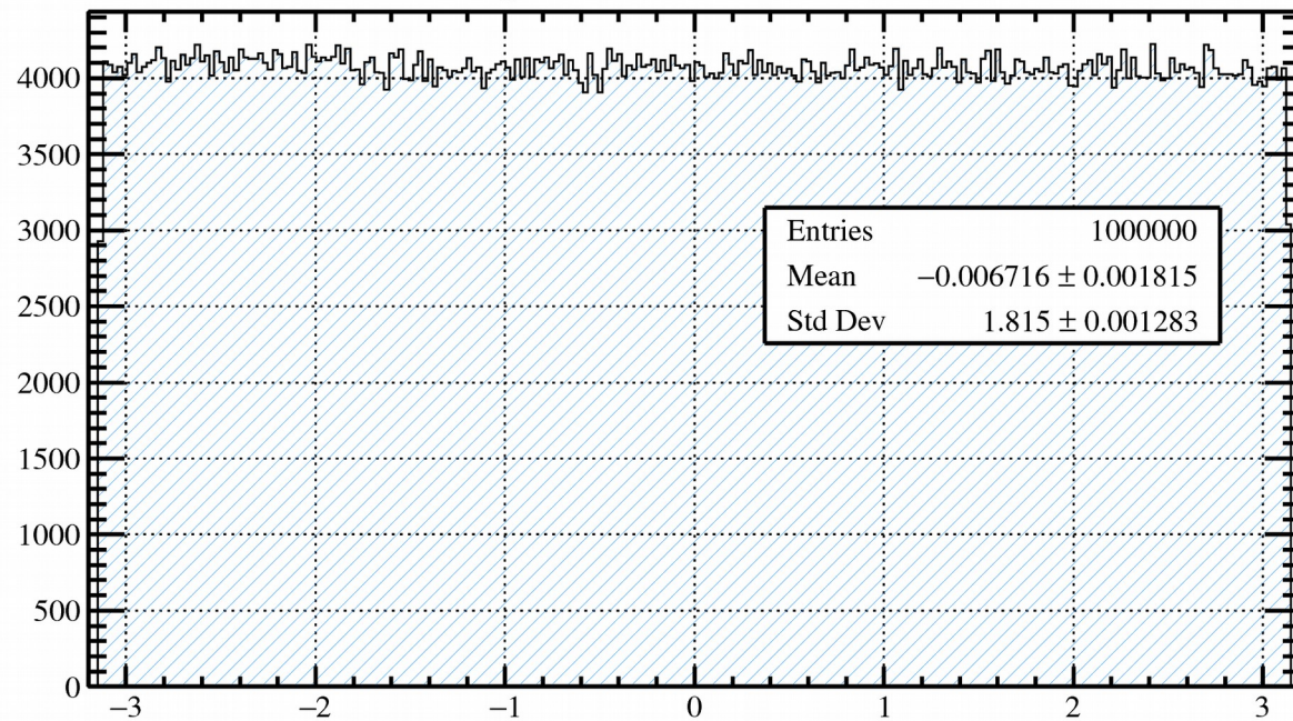
\gamma_1 Helicity Frame \phi
