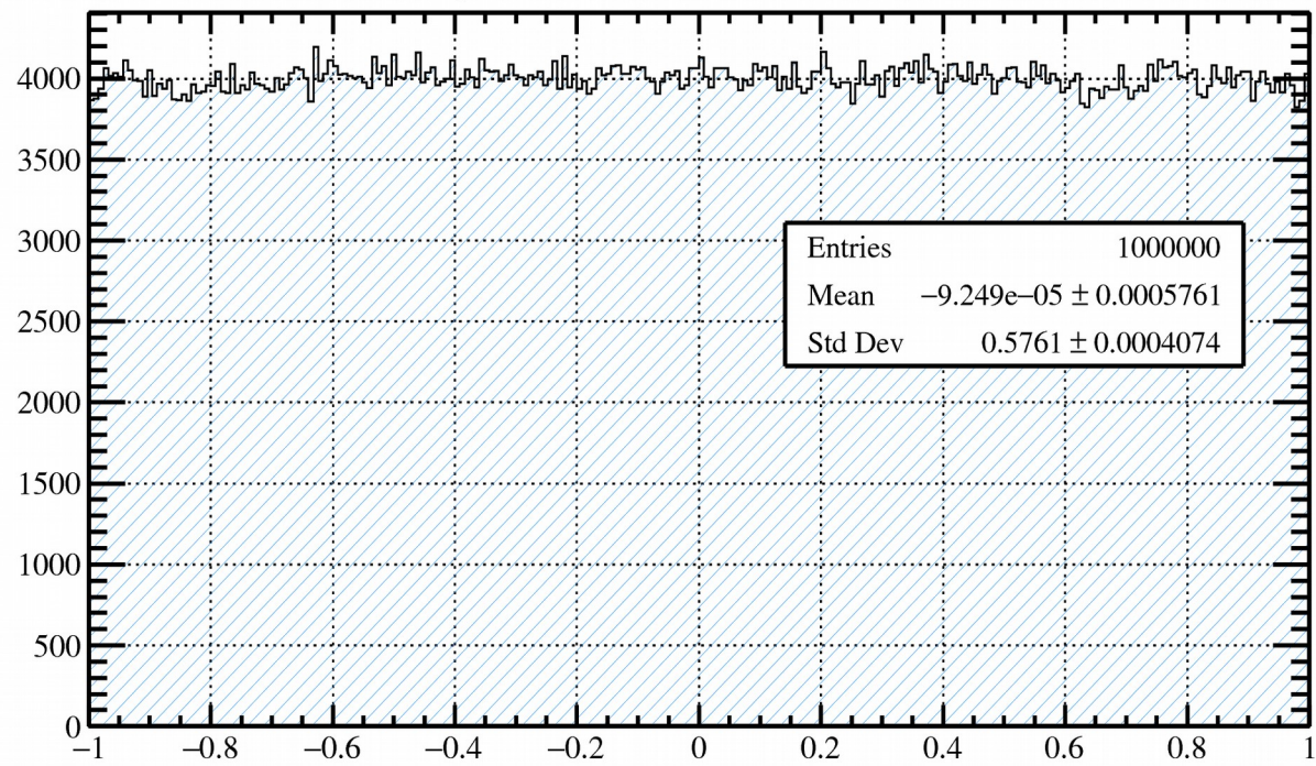
\gamma_1 Helicity Frame \cos(\theta)
