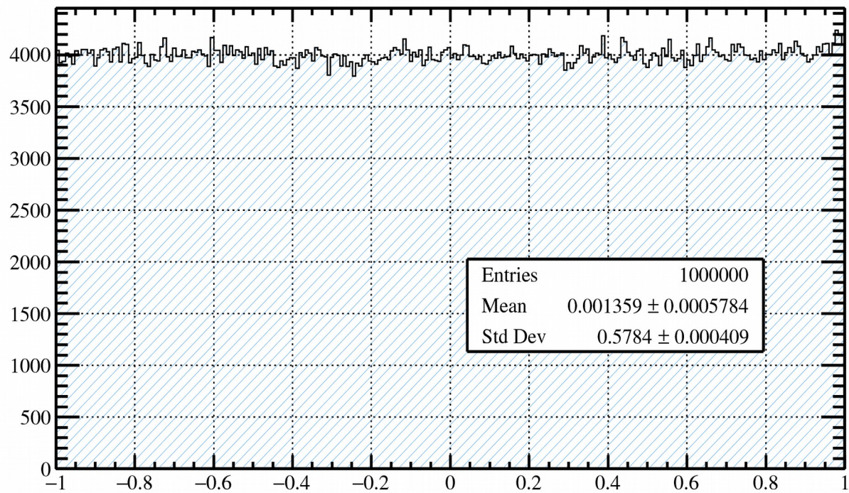
K + Helicity Frame \cos(\theta)
