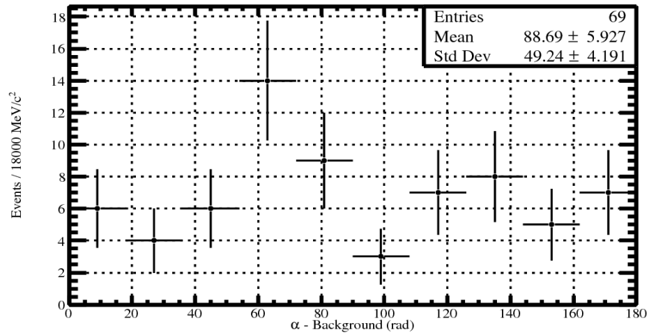
\alpha - Background (rad) [ 2\sigma ]
