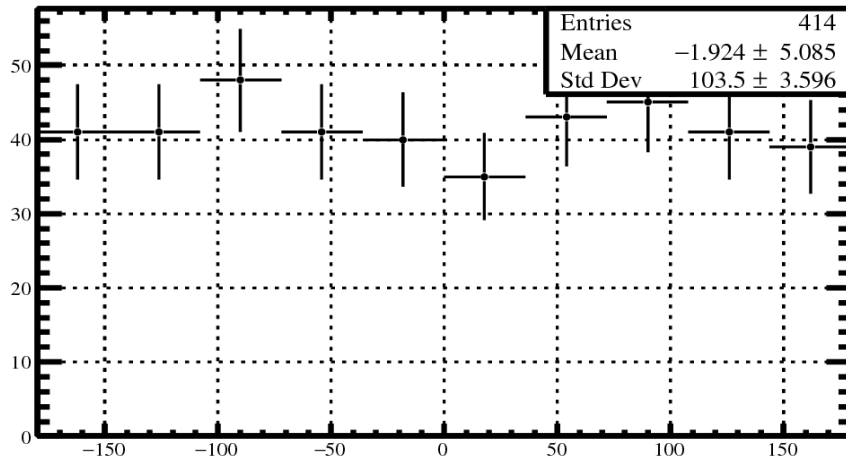
\phi GJ( \phi ) ( \alpha = 0^\circ ) - Large (deg)
