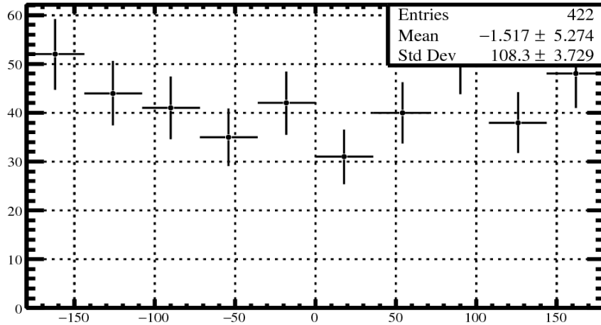
\phi GJ( \phi ) ( \alpha = \pm 90^\circ ) - Large (deg)
