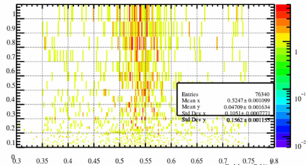
g1g2 Mass Vs BG CL
