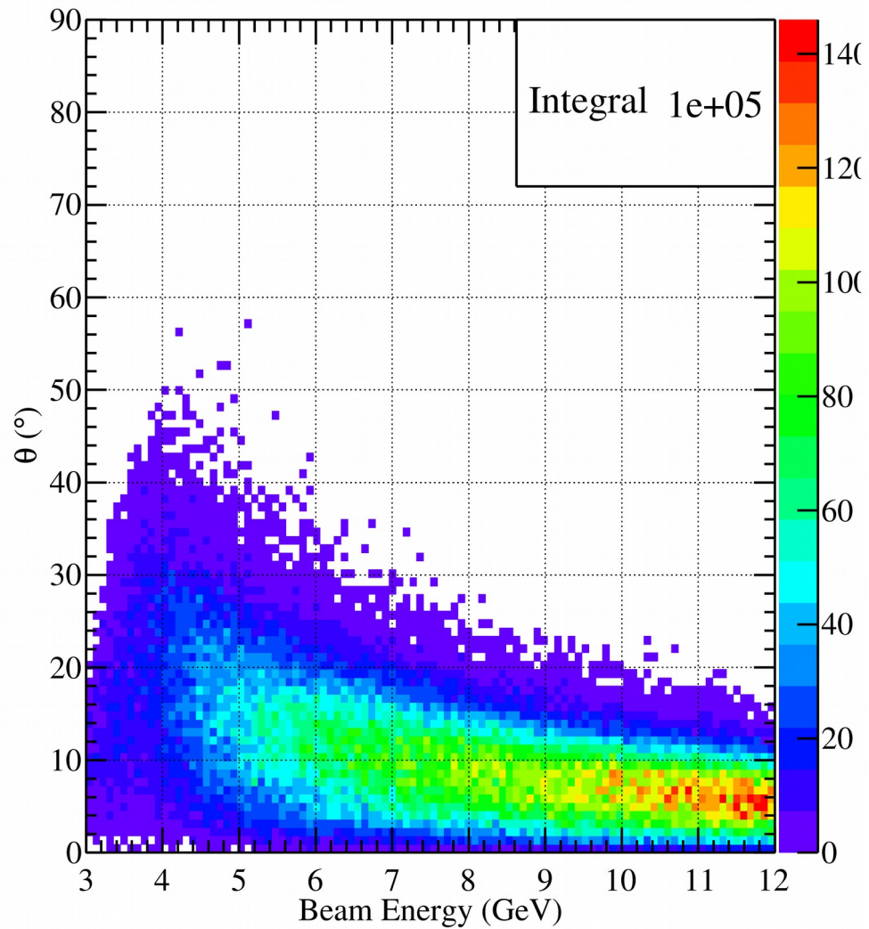
Beam Energy Vs \theta : Generated Monte Carlo
