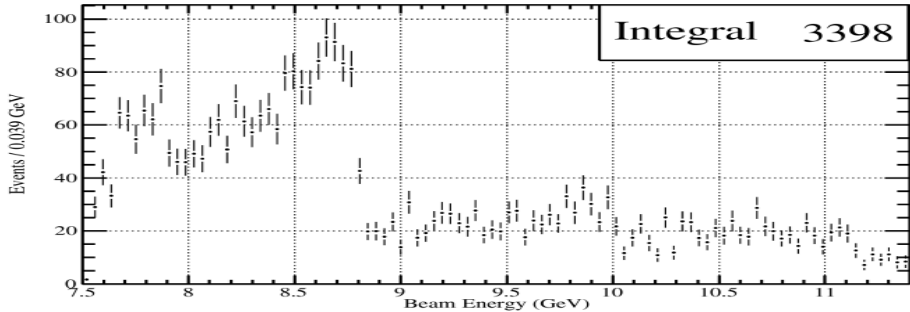
Beam Energy - Signal
