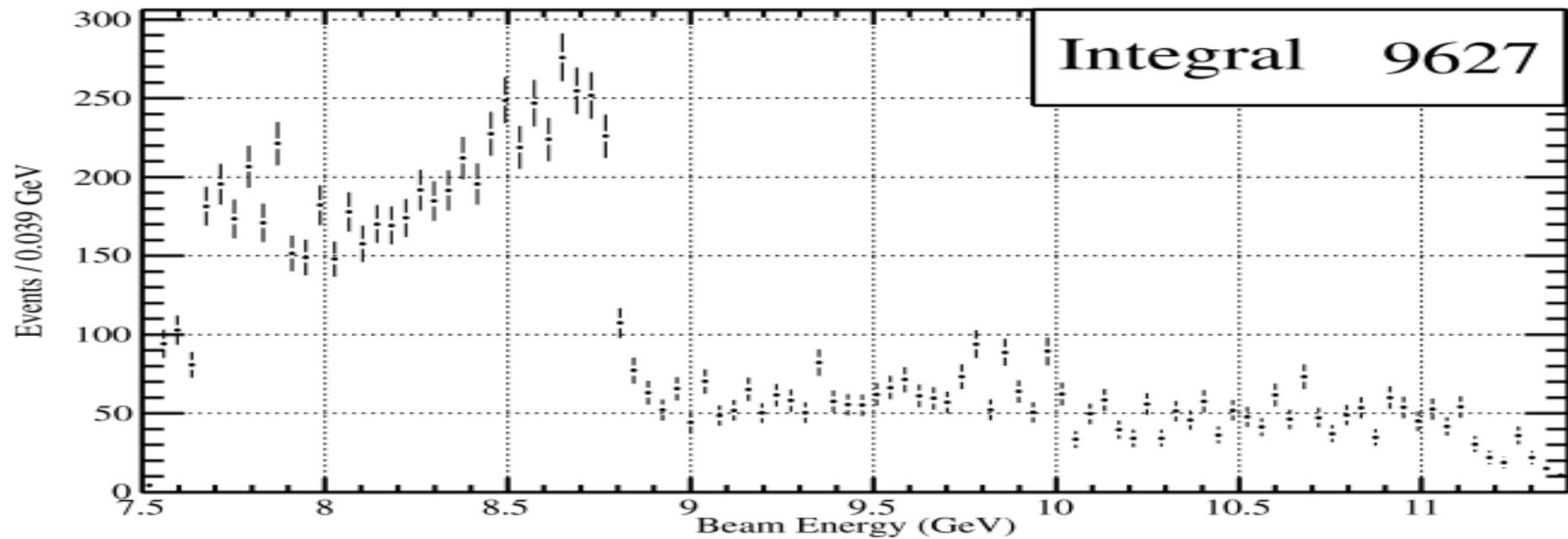
Beam Energy - Background
