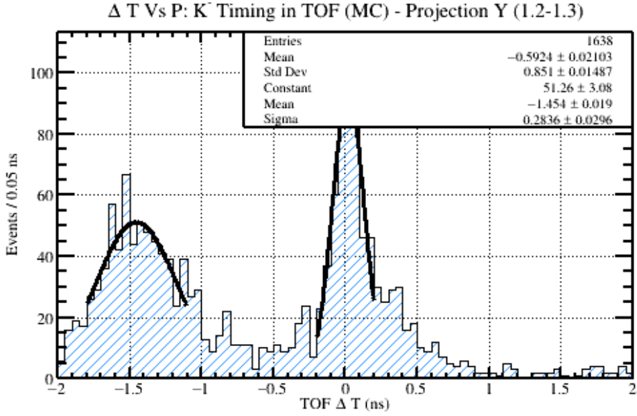
Figure 26: A projection of the statistics from Figure [25] onto the vertical (timing) axis between the momentum range of 1.2-1.3 GeV/C. This projection range is one out of many that were studied from Figure [25]. The purpose of this study is to determine the amount of pion contamination in the kaon band as a function of momentum. The results of this study are provided in Figure [27]. Lastly, two Gaussian fits were performed on this data. The mean and width of these Gaussian fits are recorded in Figure [27] for each momentum range.
