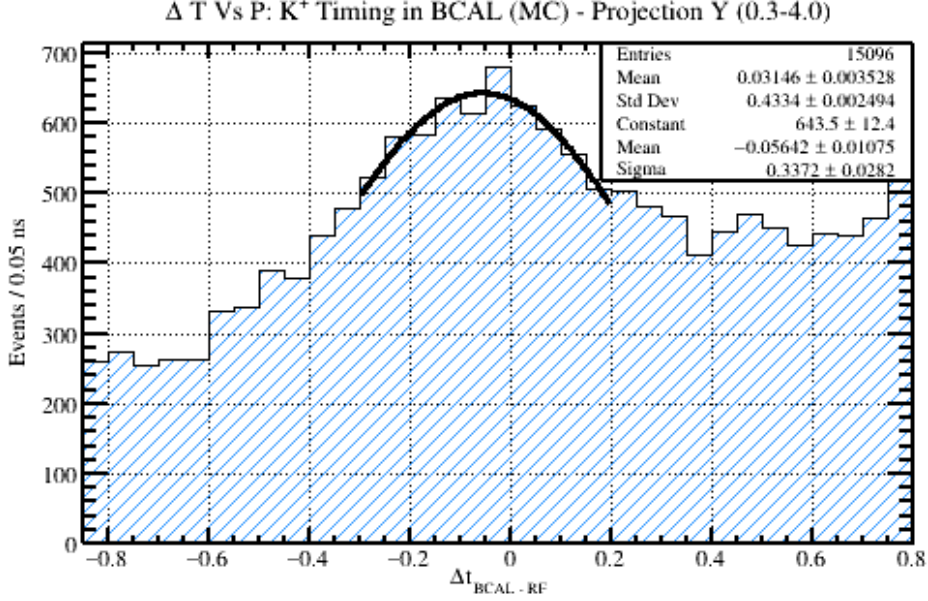
Figure 15: A projection of the statistics from Figure [14] onto the vertical (timing) axis between the momentum range of 0.3-4.0 GeV/C. A Gaussian fit was performed and is included in the figure where the mean and width of the distribution are given in the legend. The distortion of statistics towards the higher timing differences is due to protons included in this Monte Carlo study.
