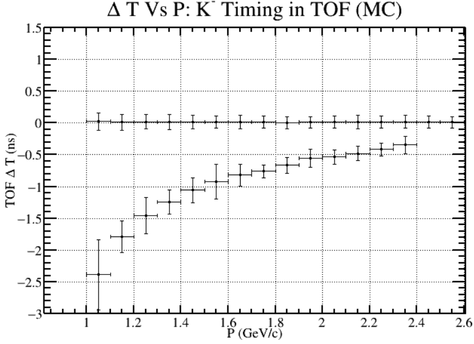
Figure 27: The image above is the result of the timing study performed on Figure [25]. Using that figure, a number of projection histograms were fit using different momentum ranges. An example of one of these fits is given in Figure [26]. The data points close to 0 \Delta T correspond to the Gaussian fits performed on the kaon signal, and the data points that approach that band from the bottom correspond to the Gaussian fits performed on the pion signal. The horizontal position of each point is in the middle of the projection range, and the vertical position of each point was assigned based on the mean value of the Gaussian fit for each particle. The horizontal error bars are the size of the projection range, which is always 0.1 GeV/c. The vertical error bars are determined by the width of the Gaussian fits.
