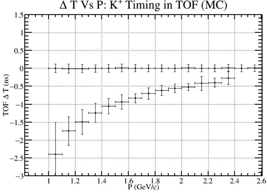
Figure 20: The image above is the result of the timing study performed on Figure [18]. Using that figure, a number of projection histograms were fit using different momentum ranges. An example of one of these fits is given in Figure [19]. The data points close to 0 \Delta T correspond to the Gaussian fits performed on the kaon signal, and the data points that approach that band from the bottom correspond to the Gaussian fits performed on the pion signal. The horizontal position of each point is in the middle of the projection range, and the vertical position of each point was assigned based on the mean value of the Gaussian fit for each particle. The horizontal error bars are the size of the projection range, which is always 0.1 GeV/c. The vertical error bars are determined by the width of the Gaussian fits.
