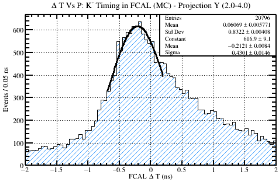
Figure 24: A projection of the statistics from Figure [23] onto the vertical (timing) axis between the momentum range of 2.0-4.0 GeV/C. This projection range was chosen so that the distortion from the lower pion band was minimized. A Gaussian fit was performed and is included in the figure where the mean and width of the distribution are given in the legend.
