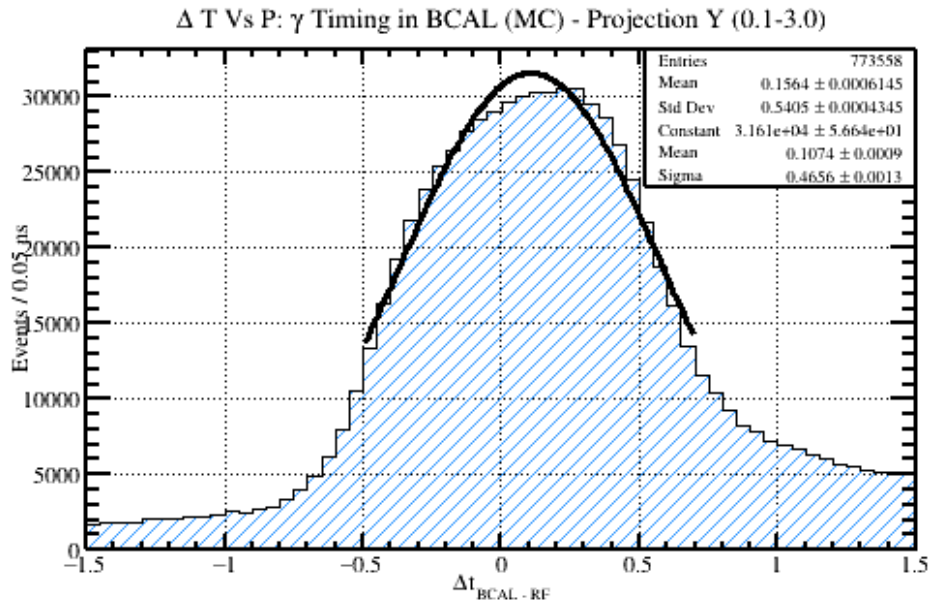
Figure 29: A projection of the statistics from Figure [28] onto the vertical (timing) axis between the momentum range of 0.1-3.0 GeV/C. A Gaussian fit was performed and is included in the figure where the mean and width of the distribution are given in the legend.
