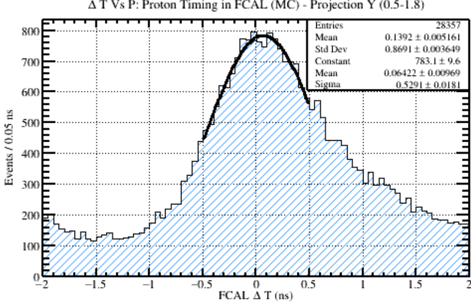
Figure 11: A projection of the statistics from Figure [10] onto the vertical (timing) axis between the momentum range of 0.5-1.8 GeV/C. This projection range was chosen so that the distortion from the lower kaon band was minimized. A Gaussian fit was performed and is included in the figure where the mean and width of the distribution are given in the legend.
