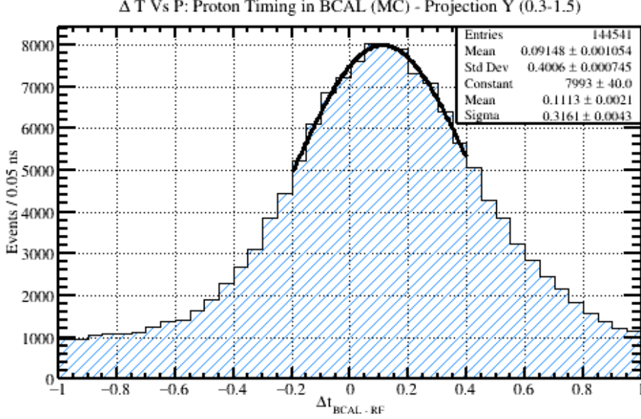
Figure 9: A projection of the statistics from Figure [8] onto the vertical (timing) axis between the momentum range of 0.3-1.5 GeV/C. This projection range was chosen so that the distortion from the lower kaon band was minimized. A Gaussian fit was performed and is included in the figure where the mean and width of the distribution are given in the legend.
