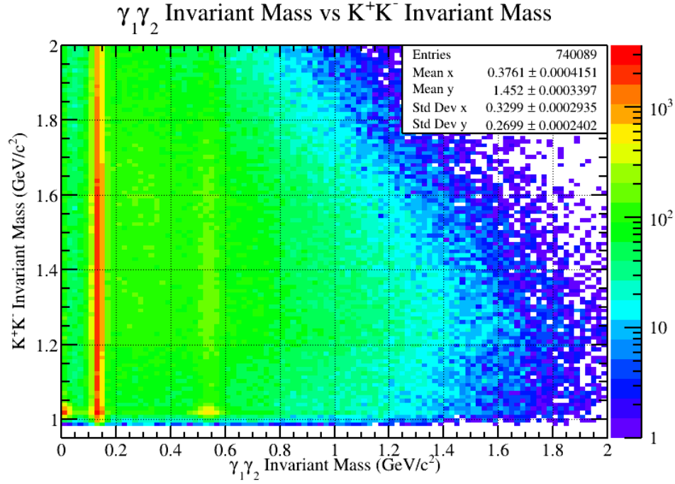
Figure 36: A two dimensional invariant mass plot with the K^+K^- invariant mass on the vertical axis, the \gamma_1\gamma_2 invariant mass on the horizontal axis, and a logarithmically scaled z axis. Some interesting features contained within the image are the clear vertical bands for the \pi^0 and \eta resonances which have large decay modes to \gamma\gamma final states. In addition, one can also observe a horizontal band slightly above 1 \frac{GeV}{c^2} which corresponds to the \phi meson decaying to a K^+K^- final state.
