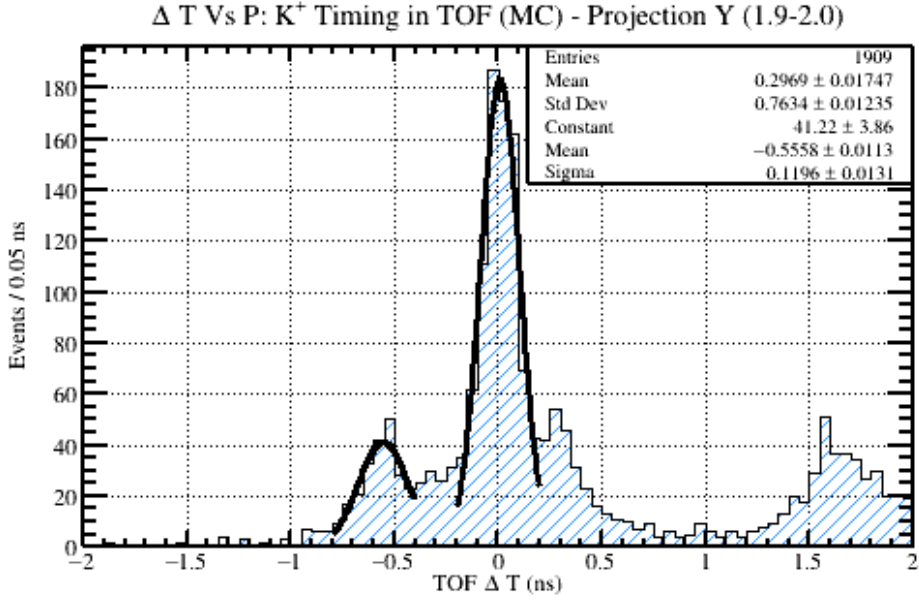
Figure 19: A projection of the statistics from Figure [18] onto the vertical (timing) axis between the momentum range of 1.9-2.0 GeV/C. This projection range is one out of many that were studied from Figure [18]. The purpose of this study is to determine the amount of pion contamination in the kaon band as a function of momentum. The results of this study are provided in Figure [20]. Lastly, two Gaussian fits were performed on this data. The mean and width of these Gaussian fits are recorded in Figure [20] for each momentum range.
