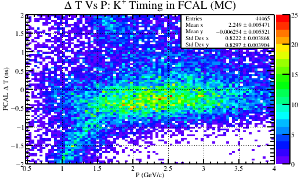
Figure 16: A timing plot for generated K^+ after reconstruction. The horizontal axis is the reconstructed momentum of the K^+ and the vertical axis is the timing difference between the FCAL and RF. The curved band that appears below the K^+ band around 1.5 GeV/c and lower comes from \pi^+ . Although pions were not explicitly generated, the computer program hdgeant (derived from geant) allows for some fraction of kaons to decay weakly while in flight; resulting in an observed pions.
