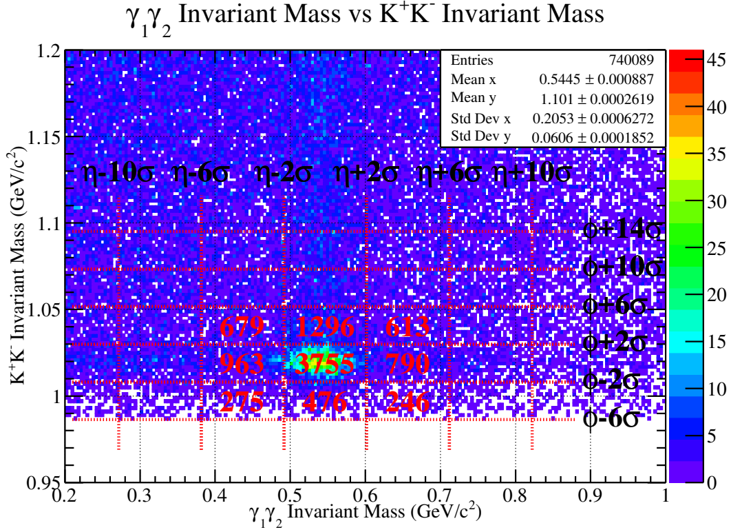
Figure 5.7: This figure shows the total number of counts in each box. To be clear, the numbers in each are do not represent the total number of events, but rather the precise amount of statistics contained. Upon inspection, one can see evidence of \phi\eta correlation, which is explained in the Conclusion section.
