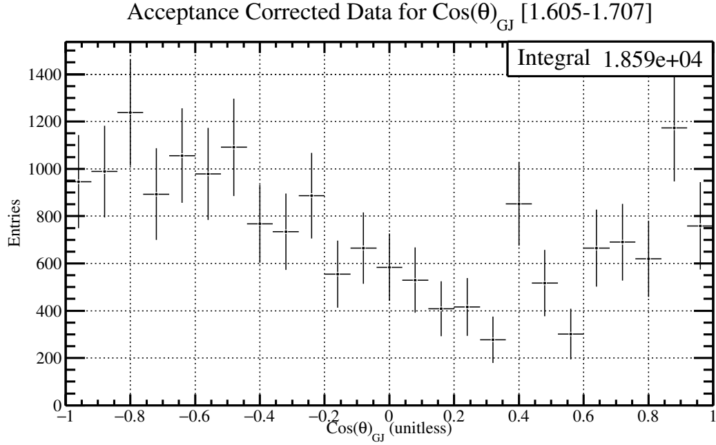
Figure 5.48: The \cos(\theta)_{GJ} distribution for \phi\eta invariant mass between 1.605-1.707 \text{GeV}/c^2 with the acceptance correction factors described in Figure [5.26].
