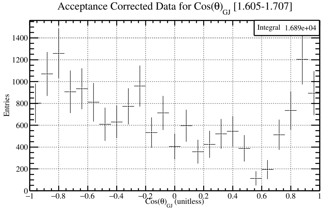
Figure 5.34: The \cos(\theta)_{GJ} distribution for \phi\eta invariant mass between 1.605-1.707 \text{GeV}/c^2 with the acceptance correction factors described in Figure [5.26].
