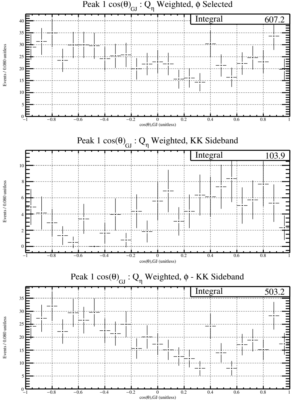
Figure 5.45: The \cos(\theta)_{GJ} distribution for \phi\eta invariant mass between 1.605-1.707 GeV/c^2 , not acceptance corrected.
