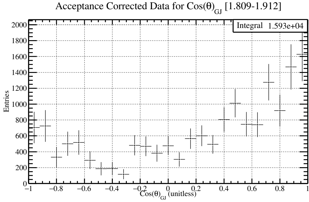
Figure 5.35: The \cos(\theta)_{GJ} distribution for \phi\eta invariant mass between 1.809-1.912 \text{GeV}/c^2 with the acceptance correction factors described in Figure [5.27].
