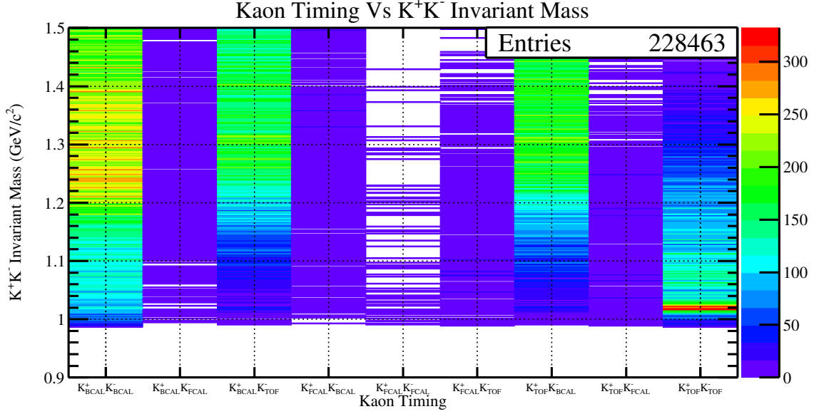
Figure 4.35: A two dimensional color histogram of the K^+K^- invariant mass versus the timing detectors for the kaons.
