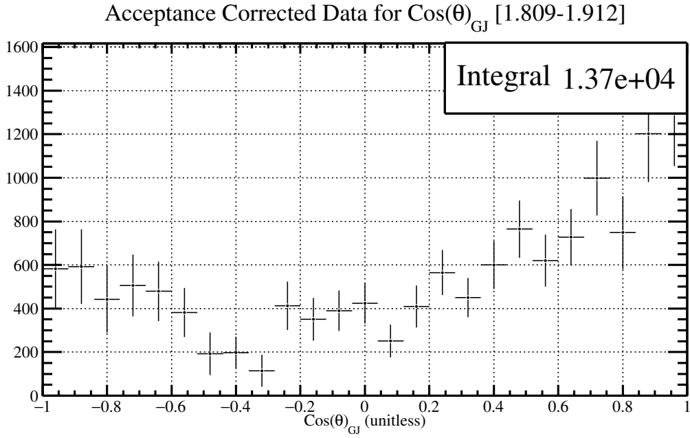
Figure 5.55: The \cos(\theta)_{GJ} distribution for \phi\eta invariant mass between 1.809-1.912 \text{GeV}/c^2 with the acceptance correction factors described in Figure [5.27].
