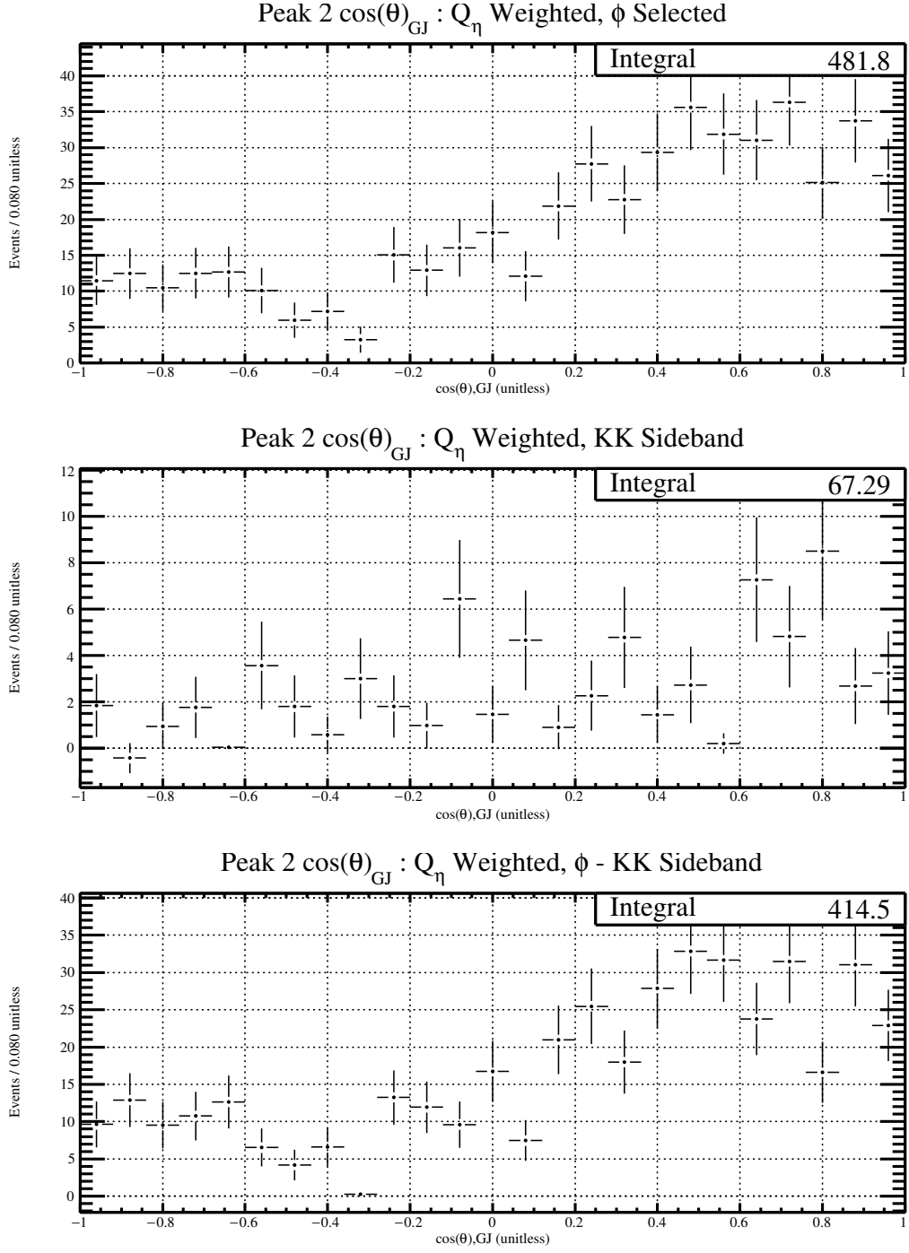
Figure 5.46: The \cos(\theta)_{GJ} distribution for \phi\eta invariant mass between 1.809-1.912 GeV/c^2 , not acceptance corrected.
