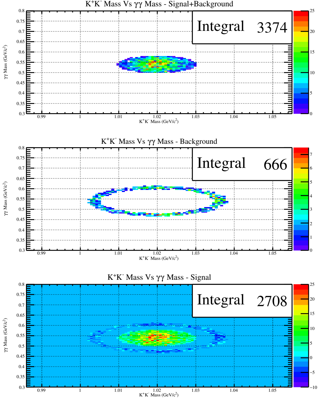
Figure 5.29: The K^+K^- invariant mass Vs \gamma\gamma invariant mass showing the elliptical mass selection method. The upper most histogram shows the ellipse which selects the \phi\eta intersection region, described by Equation 5.18. The middle histogram shows the ring which selects the background and is described by Equation 5.21. The bottom most histogram shows the difference between the upper and middle histograms.
