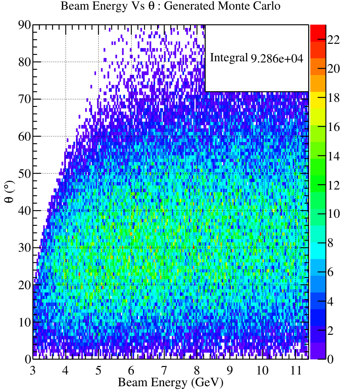
Figure 5.20: The angle of the \eta meson with respect to the beam direction in the lab frame versus the beam energy for \gamma p \rightarrow N^* \phi ; N^* \rightarrow p \eta Monte Carlo sample.
