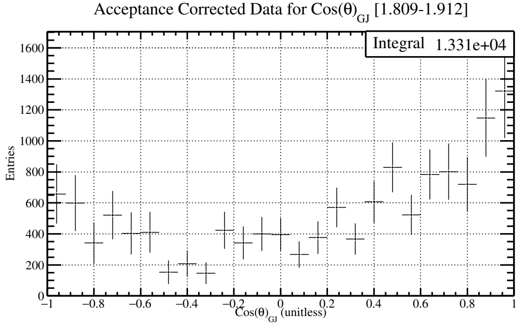
Figure 5.42: The \cos(\theta)_{GJ} distribution for \phi\eta invariant mass between 1.809-1.912 \text{GeV}/c^2 with the acceptance correction factors described in Figure [5.27].
