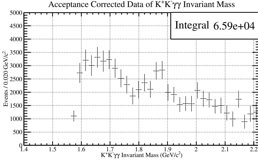
Figure 5.40: The K^+K^-\gamma\gamma invariant mass spectrum with all signal events weighted by Q_\phi , and the \eta is selected by side-band subtraction. The spectrum is acceptance corrected as described by Figure [5.25]. The range of the distribution has been changed due to the large error bars at high \phi\eta invariant mass values.
