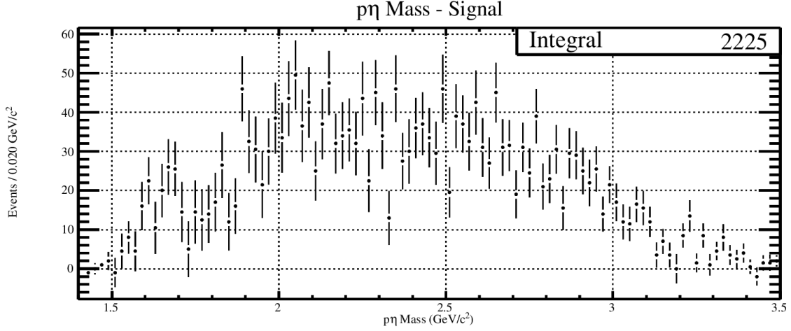
Figure 5.23: The p\gamma\gamma invariant mass for the Elliptical Subtraction method (Subsec: 5.5.1) after a \theta cut of 18^\circ .
