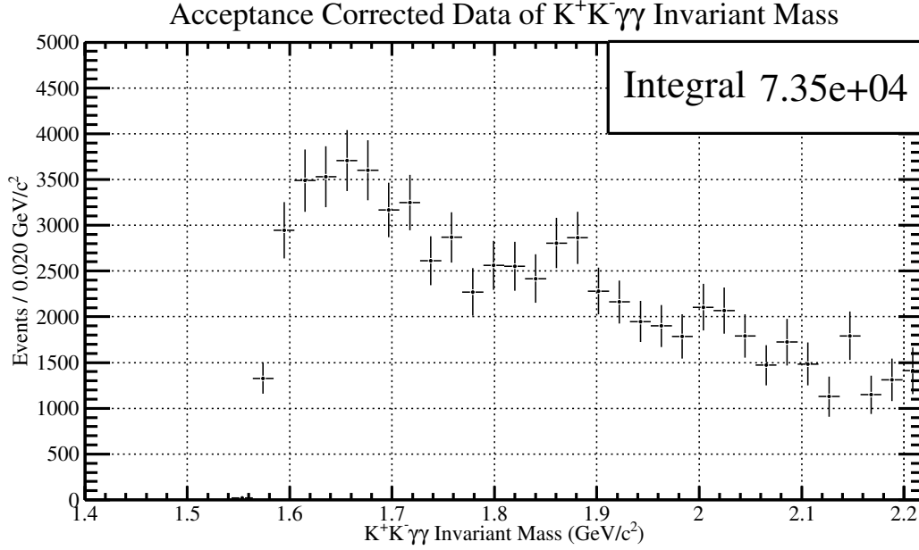
Figure 5.53: he K^+K^-\gamma\gamma invariant mass spectrum with all signal events weighted by Q_{\phi\eta} . The spectrum is acceptance corrected as described by Figure [5.25]. The range of the distribution has been changed due to the large error bars at high \phi\eta invariant mass values.
