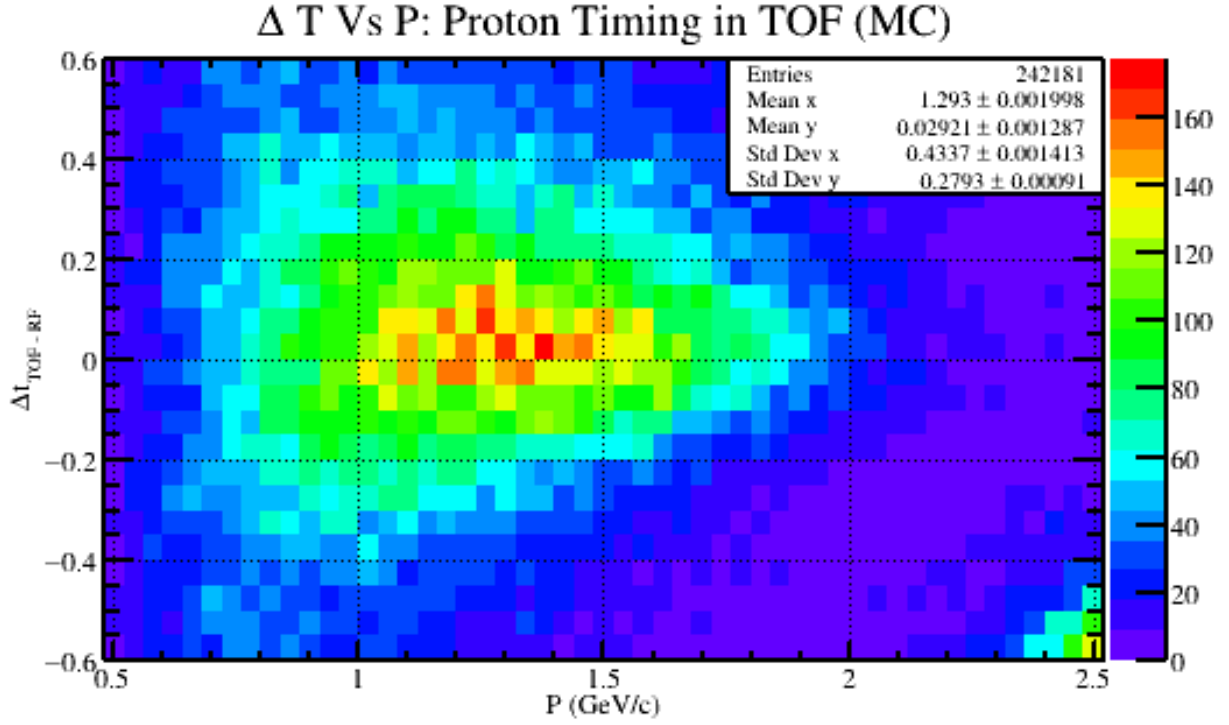
Figure 4.9: A timing plot for accepted recoil protons from the generated reaction \gamma p \rightarrow pX ; X \rightarrow \phi\eta ; \phi \rightarrow K^+K^- ; \eta \rightarrow \gamma\gamma . The horizontal axis is the reconstructed momentum of the proton and the vertical axis is the timing difference between the TOF and RF. The enhancement of statistics in the lower right portion of the plot comes from miss identified kaons that are also present in the generated Monte Carlo, specifically Figure [4.2a] and Figure [4.2b].
