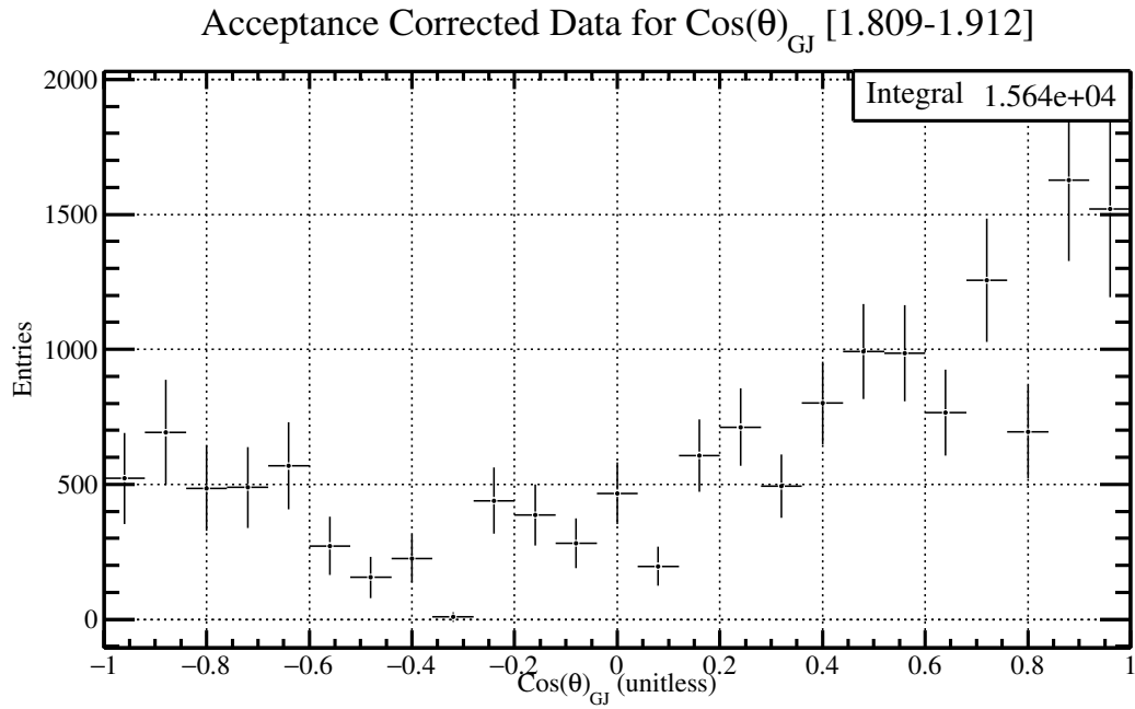
Figure 5.49: The \cos(\theta)_{GJ} distribution for \phi\eta invariant mass between 1.809-1.912 \text{GeV}/c^2 with the acceptance correction factors described in Figure [5.27].
