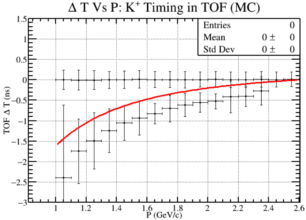
Figure 4.33: A histogram which provides the strangeness conservation cut used for kaons that are detected by the Time of Flight detector. This is identical to Figure 4.18, except that it includes a red line which represents Equation 4.3, with a timing shift of 0.2 ns.
