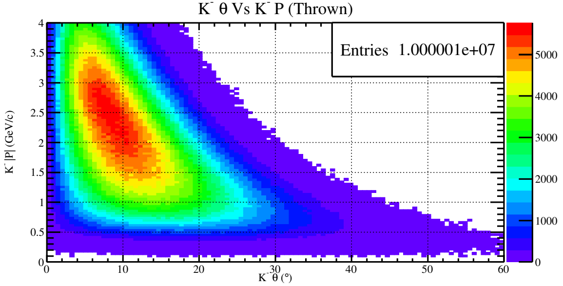
Figure 3.4: A two dimensional histogram which includes the thrown kinematic information of the generated K^- . In the histogram, the horizontal axis represents the generated \theta angle in the lab frame, and the vertical axis represents the generated momentum magnitude in the lab frame.
