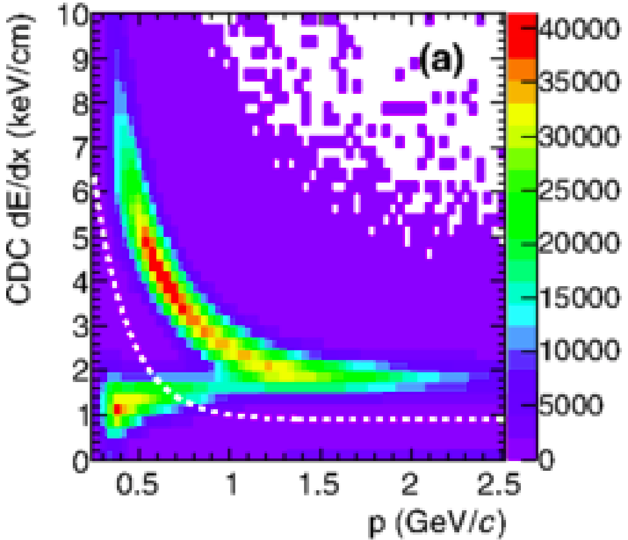
Figure 4.3: A figure which shows the energy lost in the Central Drift Chamber on the vertical axis, and the reconstructed momentum on the horizontal axis. At lower momentum, a proton band can be seen rising sharply towards higher energy loss values. Also contained within the figure is a white dashed line which represents the cut value used to identify slower moving protons. The horizontal band which deviates from the proton band at low momentum comes from positively charged pions and kaons.
