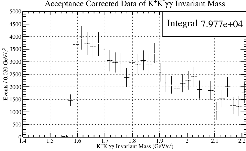
Figure 5.47: The K^+K^-\gamma\gamma invariant mass spectrum with all signal events weighted by Q_\eta , and the \phi is selected by side-band subtraction. The spectrum is acceptance corrected as described by Figure [5.25]. The range of the distribution has been changed due to the large error bars at high \phi\eta invariant mass values.
