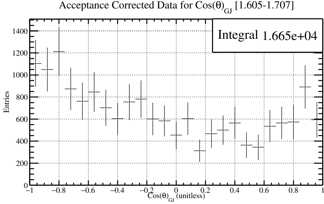
Figure 5.41: The \cos(\theta)_{GJ} distribution for \phi\eta invariant mass between 1.605-1.707 \text{GeV}/c^2 with the acceptance correction factors described in Figure [5.26].
