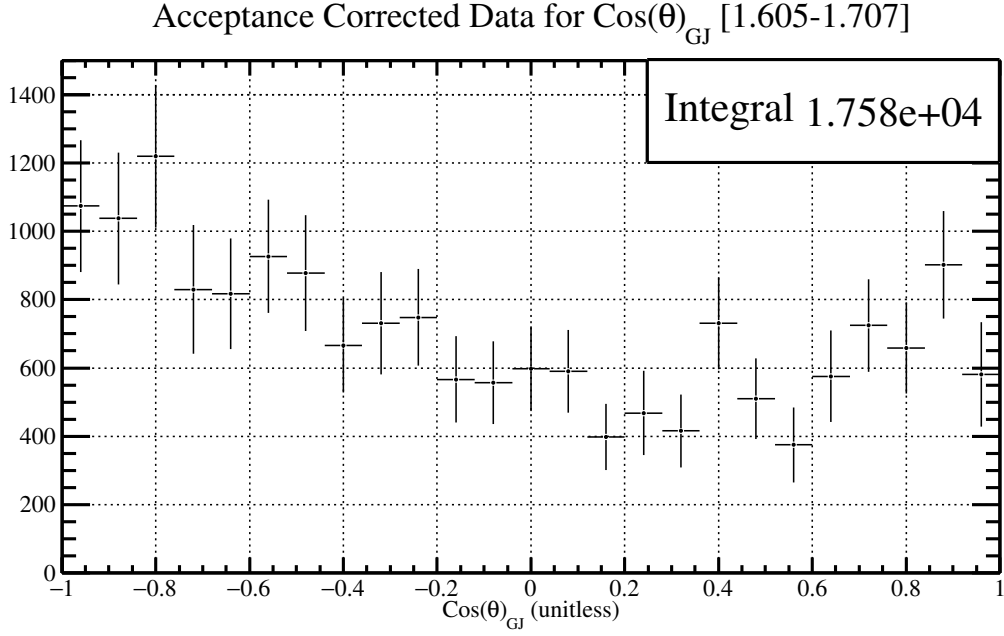
Figure 5.54: The \cos(\theta)_{GJ} distribution for \phi\eta invariant mass between 1.605-1.707 \text{GeV}/c^2 with the acceptance correction factors described in Figure [5.26].
