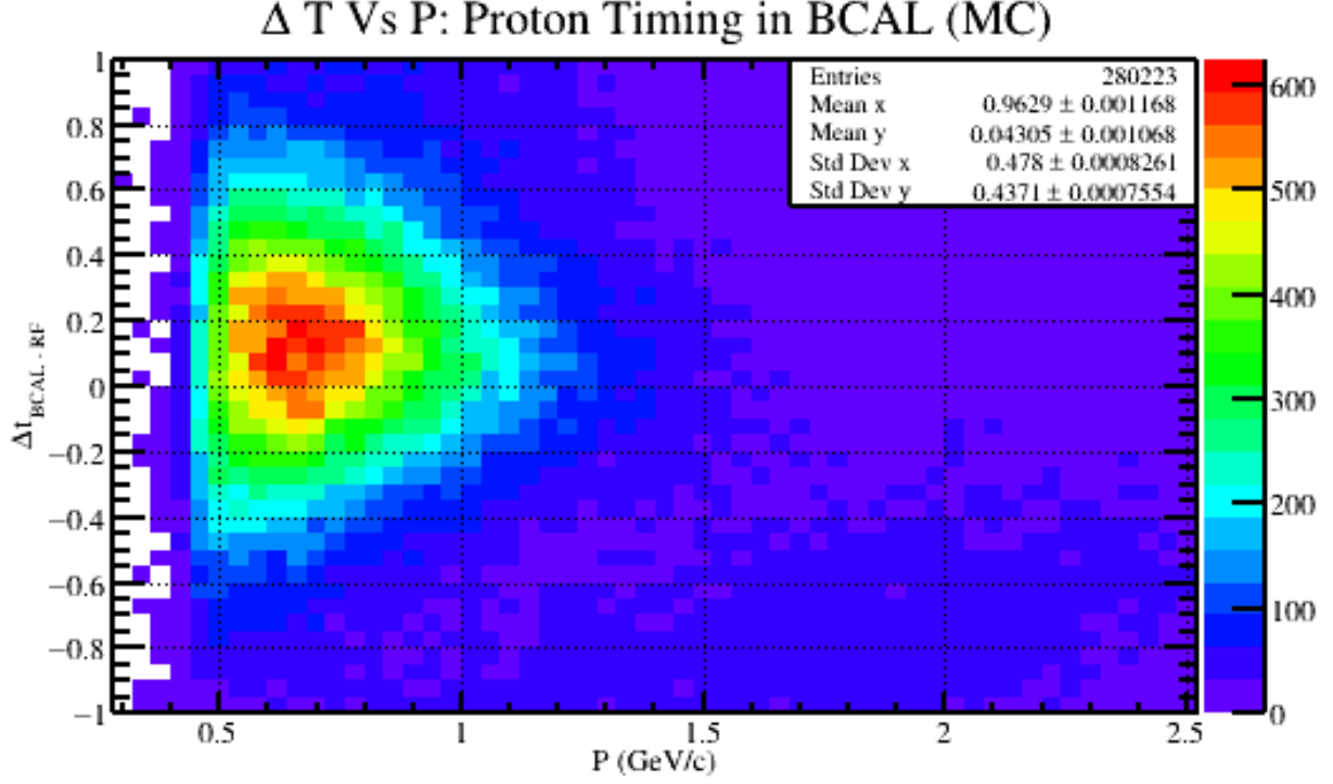
Figure 4.5: A timing plot for accepted recoil protons from the generated reaction \gamma p \rightarrow pX ; X \rightarrow \phi\eta ; \phi \rightarrow K^+K^- ; \eta \rightarrow \gamma\gamma . The horizontal axis is the reconstructed momentum of the recoil proton and the vertical axis is the timing difference between the BCAL and RF. The enhancement of statistics in the lower right portion of the plot comes from miss identified kaons that are also present in the accepted Monte Carlo.
