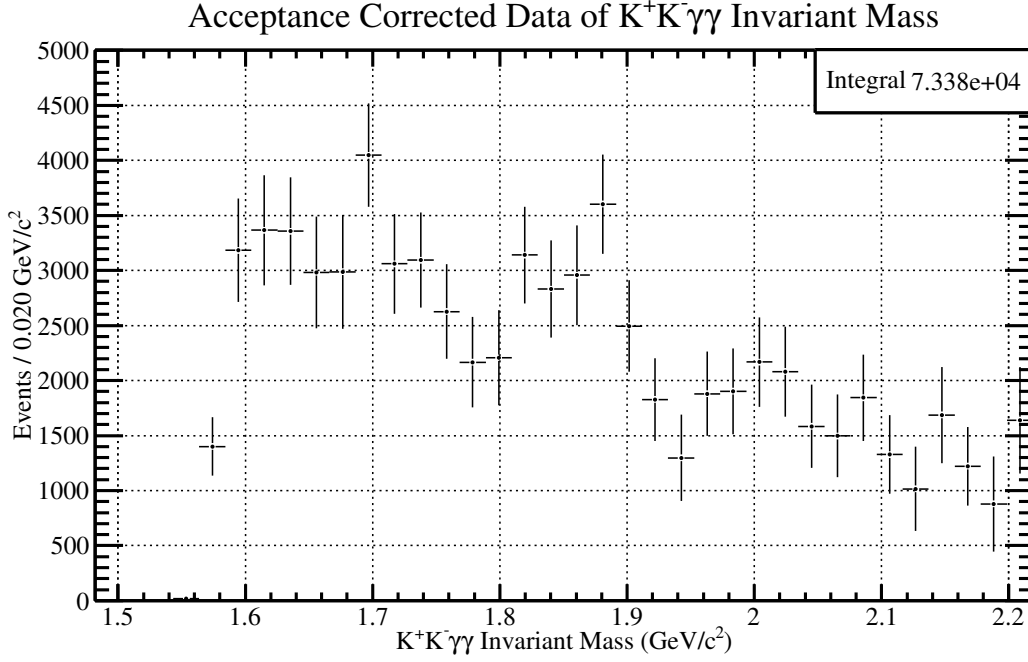
Figure 5.33: The signal \phi\eta invariant mass for elliptical mass selection with the acceptance correction factors described in Figure [5.25]. The range of the distribution has been changed due to the large error bars at high \phi\eta invariant mass values.
