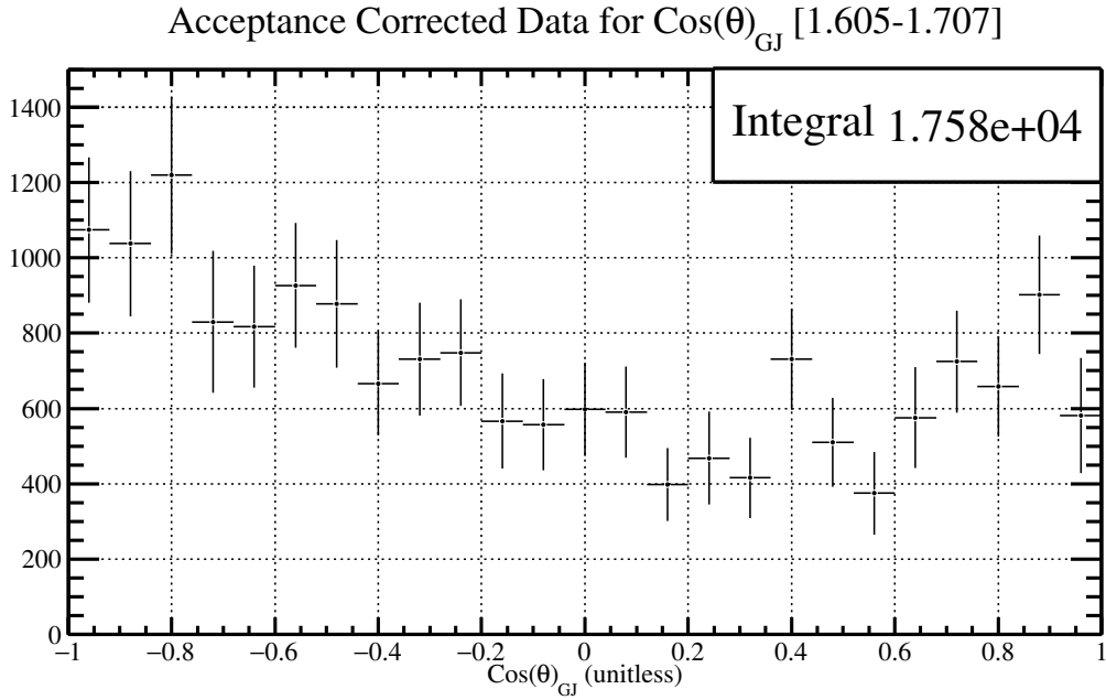
Figure 5.54: The \text{cos}(\theta)_{GJ} distribution for \phi\eta invariant mass between 1.605\text{--}1.707 \text{ GeV}/c^2 with the acceptance correction factors described in Figure [5.26].
