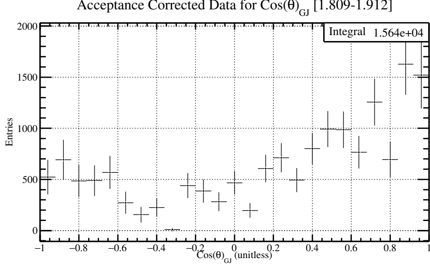
Figure 5.49: The \cos(\theta)_{GJ} distribution for \phi\eta invariant mass between 1.809-1.912 GeV/c^2 with the acceptance correction factors described in Figure [5.27].
