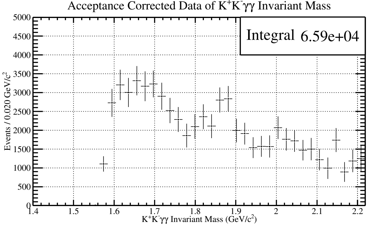
Figure 5.40: The K^+K^-\gamma\gamma invariant mass spectrum with all signal events weighted by Q_\phi , and the \eta is selected by side-band subtraction. The spectrum is acceptance corrected as described by Figure [5.25]. The range of the distribution has been changed due to the large error bars at high \phi\eta invariant mass values.
