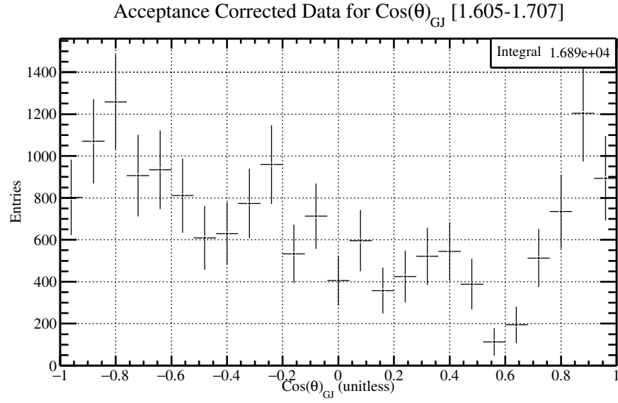
Figure 5.34: The \cos(\theta)_{GJ} distribution for \phi\eta invariant mass between 1.605-1.707 \text{GeV}/c^2 with the acceptance correction factors described in Figure [5.26].
