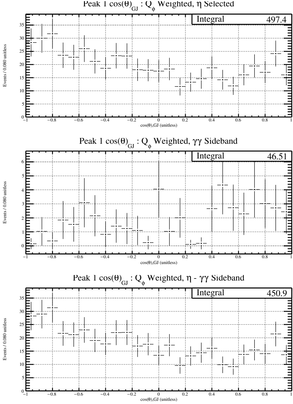
Figure 5.38: The \cos(\theta)_{GJ} distribution for \phi\eta invariant mass between 1.605 - 1.707 \text{GeV}/c^2 , not acceptance corrected.
