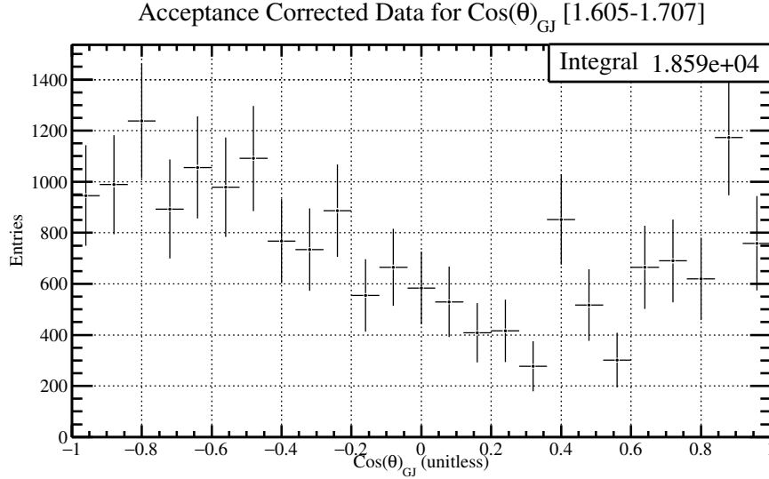
Figure 5.48: The \cos(\theta)_{GJ} distribution for \phi\eta invariant mass between 1.605-1.707 GeV/c^2 with the acceptance correction factors described in Figure [5.26].
