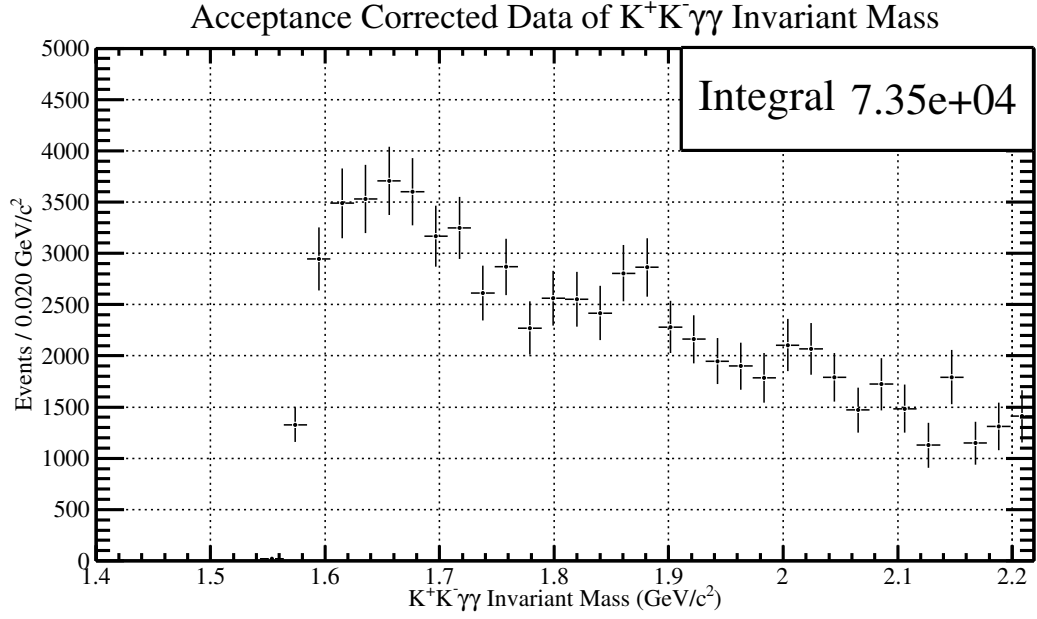
Figure 5.53: The K^+K^-\gamma\gamma invariant mass spectrum with all signal events weighted by Q_{\phi\eta} . The spectrum is acceptance corrected as described by Figure [5.25]. The range of the distribution has been changed due to the large error bars at high \phi\eta invariant mass values.
