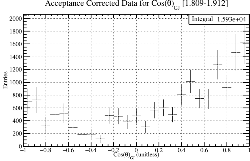
Figure 5.35: The \cos(\theta)_{GJ} distribution for \phi\eta invariant mass between 1.809-1.912 GeV/c^2 with the acceptance correction factors described in Figure [5.27].
