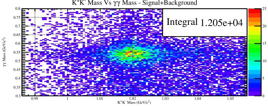
Figure 5.28: The K^+K^- invariant mass Vs \gamma\gamma invariant mass before elliptical Mass selection.
