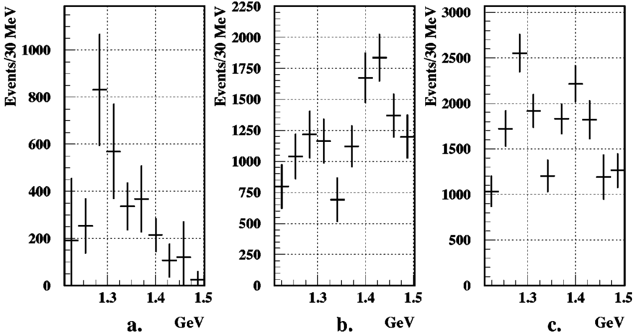
Figure 22: Fitted intensity distributions from E852 for the 0^{-+} wave [209]: (a) a_0\pi intensity, (b) \eta(\pi\pi)_S intensity, and (c) total 0^{-+} intensity. A sharp peak at about 1300 MeV/ c^2 is visible in (a), consistent with the assumption of \eta(1295) \rightarrow a_0(980)\pi .
