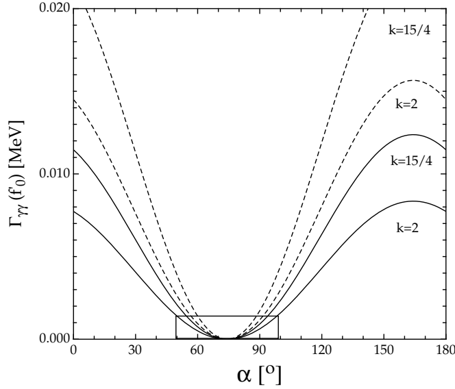
Figure 24: Predicted two-photon width for the f_0(1500) (solid curves) and f_0(1710) (dashed curves) assuming a q\bar{q} structure. The box shows the 95 % confidence-level upper limit from ALEPH for the f_0(1500) . The picture is taken from [184].
