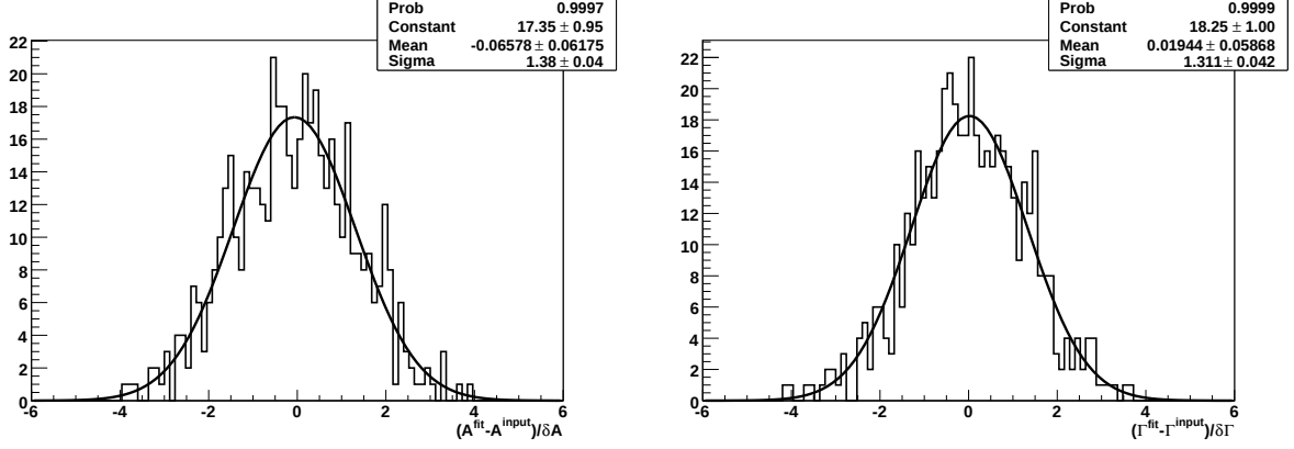
Figure 5: Distributions of (A^{fit} - A^{input})/\delta A (left) and (\Gamma^{fit} - \Gamma^{input})/\delta \Gamma (right) obtained with the sFit method, with superimposed gaussian fits, for the scenario S_m/\sigma_m = 6 , N_s = 5000 and N_b/N_s = 1.5 .
