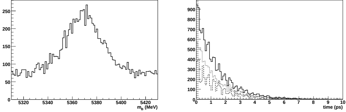
Figure 1: Distributions from a data set with S_m/\sigma_m = 6 , N_s = 5000 and N_b/N_s = 1.5 . Left: the B mass distribution; right: the total time distribution (solid), as well as the signal time distribution (dashed) and background time distribution (dot-dashed) reconstructed using the sPlot technique.
