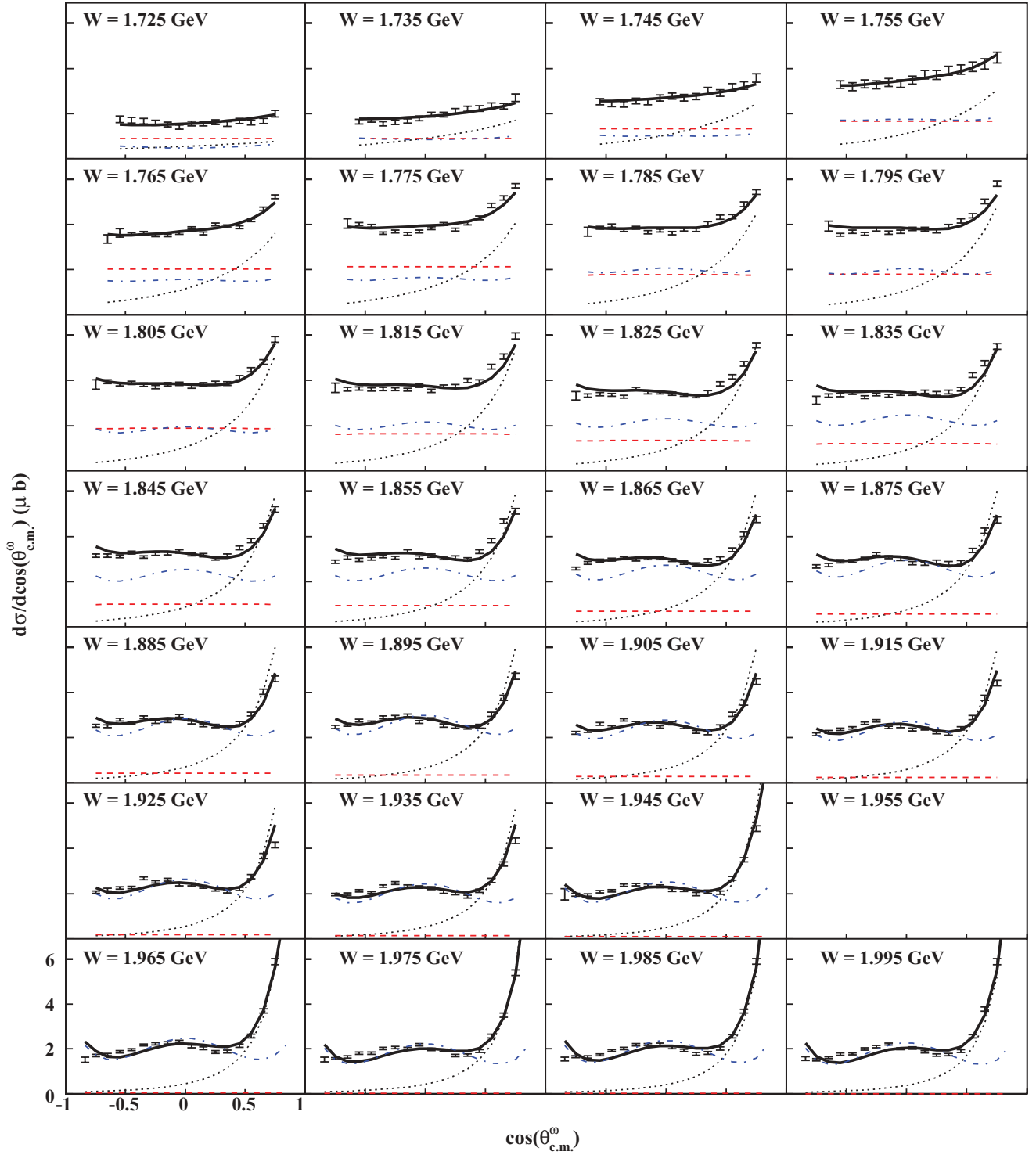
FIG. 5. (Color online) d\sigma/d\cos\theta_{\text{c.m.}}^{\omega} ( \mu\text{b} ) vs \cos\theta_{\text{c.m.}}^{\omega} : PWA results from Fit I (solid black line), compared to our measurements [11]. The individual contributions from the J^P = 3/2^- wave (red, dashed line), J^P = 5/2^+ wave (blue, dashed-dotted line), and OTL t -channel terms (dotted black line) are also shown. The lack of data reported in the W = 1.955 GeV bin is due to normalization issues [11].
