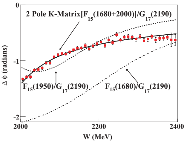
FIG. 8. (Color online) Results from Fit II: \Delta\phi = \phi_{7/2^-} - \phi_{5/2^+} (radians) vs W (MeV): The dot-dashed line is the phase motion expected using constant width Breit-Wigner distributions and the parameters quoted by the PDG for the F_{15}(1680) and G_{17}(2190) . The dashed line required the J^P = 7/2^- parameters to be within the PDG limits for the G_{17}(2190) , while allowing the J^P = 5/2^+ parameters to vary freely. The solid line used a constant width Breit-Wigner distribution for the G_{17}(2190) , but a two-pole single channel K -matrix for the J^P = 5/2^+ wave. The parameters obtained from these fits are listed in the text. The error bars are purely statistical.
