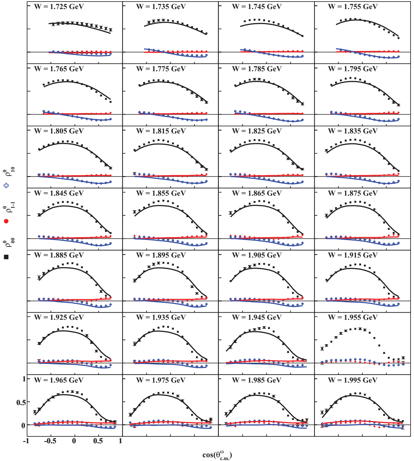
FIG. 6. (Color online) \rho_{MM'}^0 vs \cos \theta_{c.m.}^\omega : PWA results from Fit I: \rho_{00}^0 (solid black line), \rho_{1-1}^0 [solid middle (red) line], \text{Re} \rho_{10}^0 [solid bottom (blue) line], compared to our measurements [11]. The lack of a fit in the W = 1.955 GeV bin is due to normalization issues [11].
