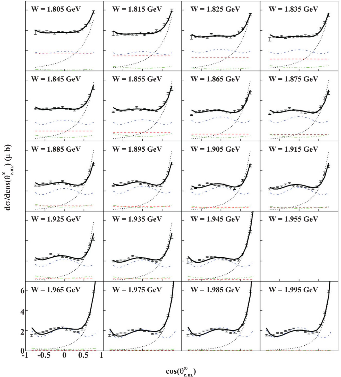
FIG. 12. (Color online) d\sigma/d\cos\theta_{\text{c.m.}}^{\omega} ( \mu\text{b} ) vs \cos\theta_{\text{c.m.}}^{\omega} : PWA results from Fit III (solid black line), compared to our measurements [11]. The individual contributions from the J^P = 3/2^- wave (red, dashed line), J^P = 5/2^+ wave (blue, dashed-dotted line), the J^P = 3/2^+ wave (green, dashed-triple-dotted line), and OTL t -channel terms (dotted black line) are also shown. The lack of data reported in the W = 1.955 GeV bin is due to normalization issues [11].
