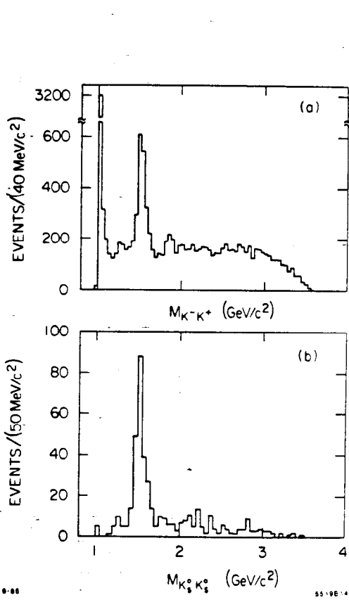
Fig. 1. The \bar{K}K mass spectra from (a) reaction (1) and (b) reaction (2).
