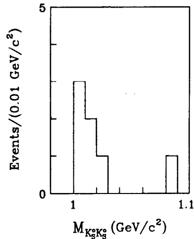
Fig. 6. The \bar{K}K threshold region of reaction (2).
