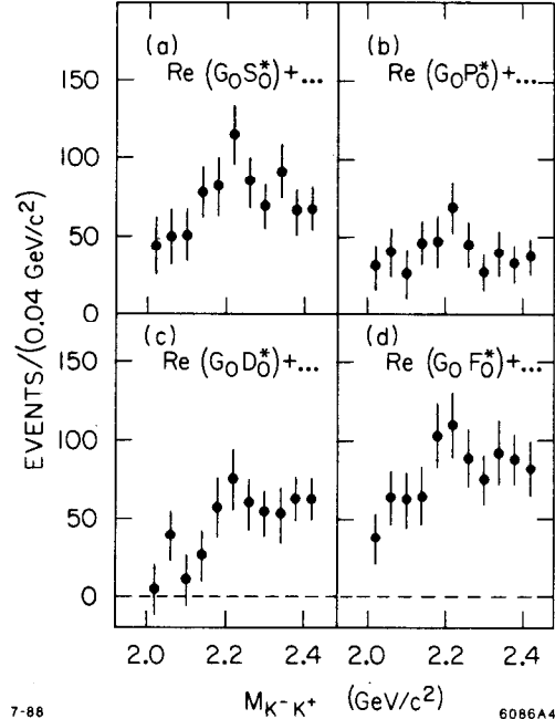
Fig. 5. Moments sums from reaction (1) dominated by leading G-wave interference terms according to the model described in the text.
