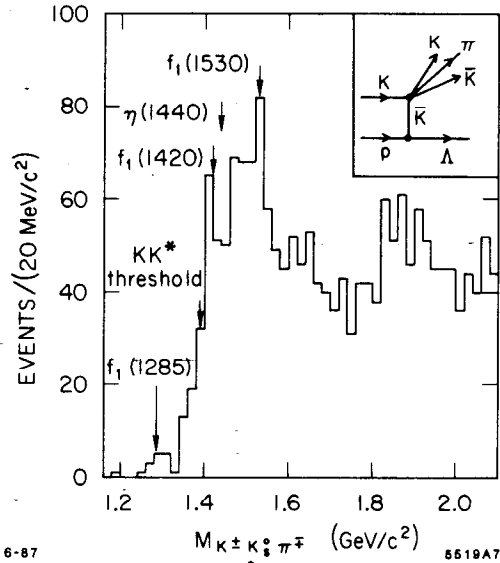
Fig. 7. The \bar{K}K\pi mass spectrum from reactions (3).
