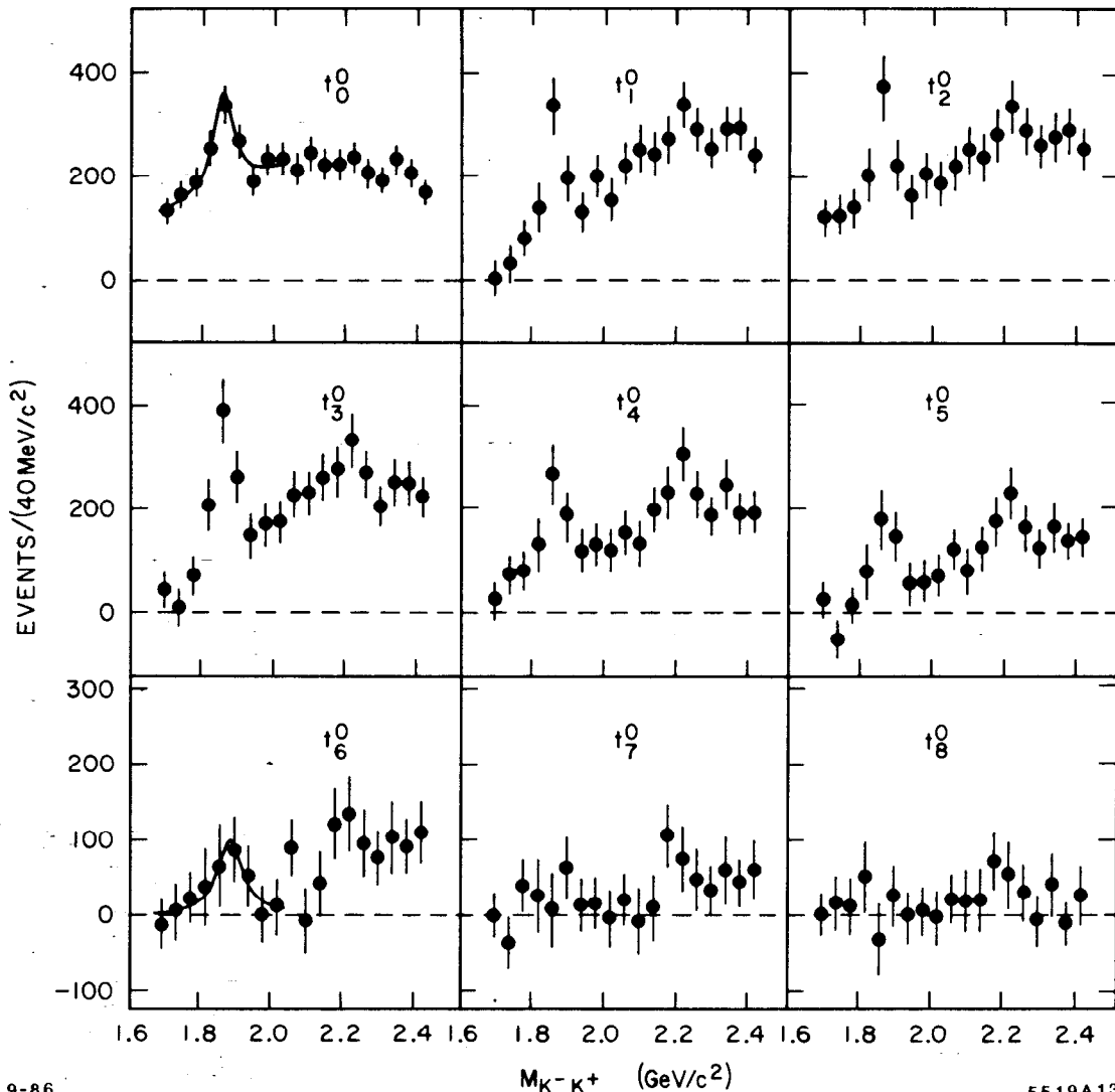
Fig. 3. The unnormalised M = 0 \bar{K}K moments from reaction (1) above the f_2'(1525) with t' < 0.2(\text{GeV}/c)^2 required.
