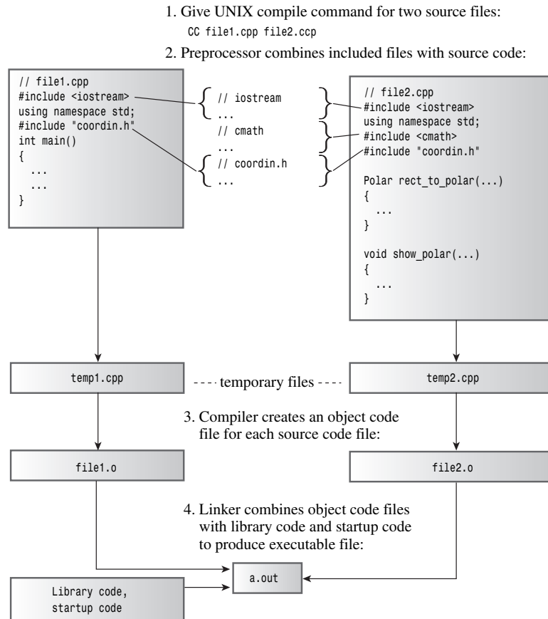
FIGURE 9.1 Compiling a multifile C++ program on a Unix system.
