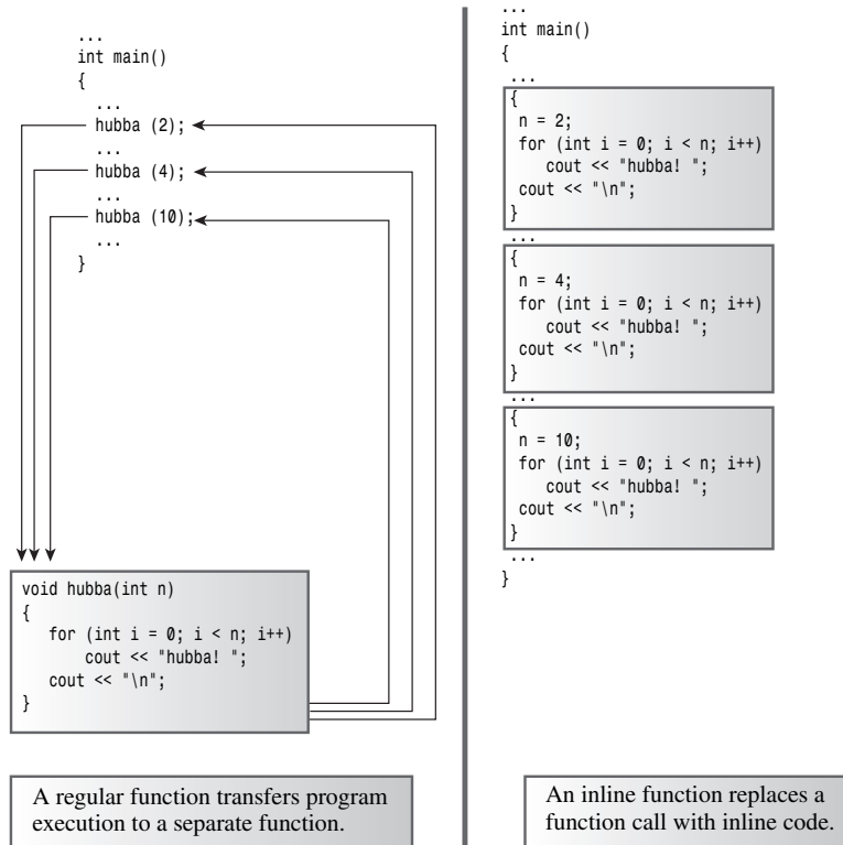
FIGURE 8.1 Inline functions versus regular functions.
