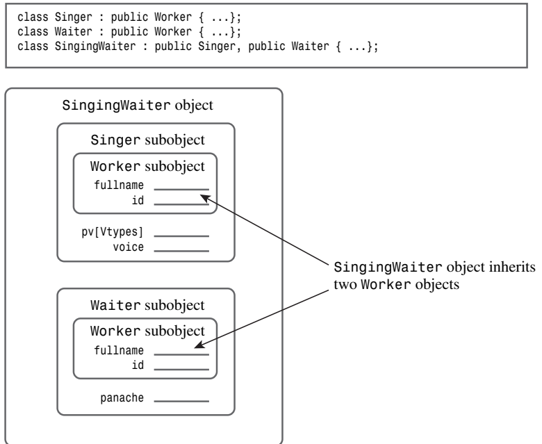
FIGURE 14.4 Inheriting two base-class objects.
