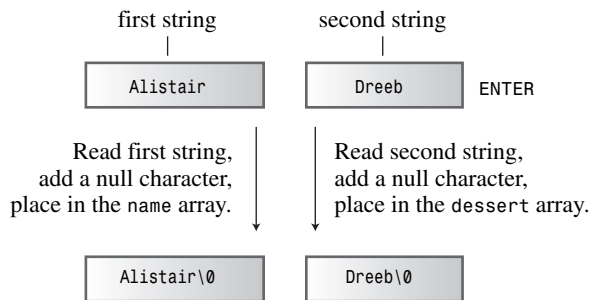
FIGURE 4.4 The cin view of string input.
