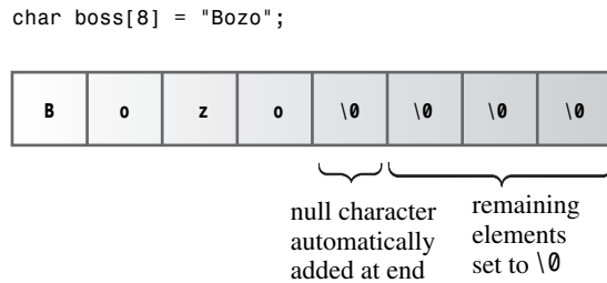
FIGURE 4.2 Initializing an array to a string.
