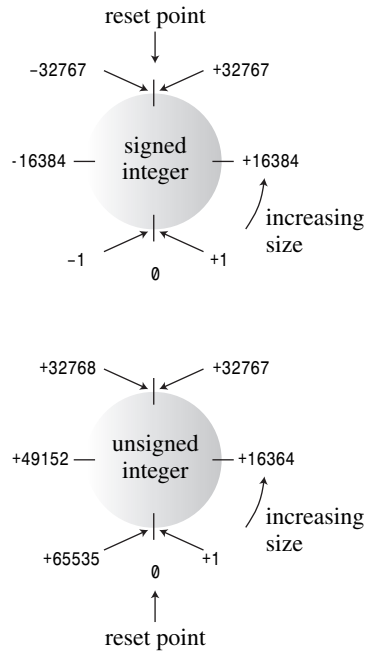
FIGURE 3.1 Typical overflow behavior for integers.
