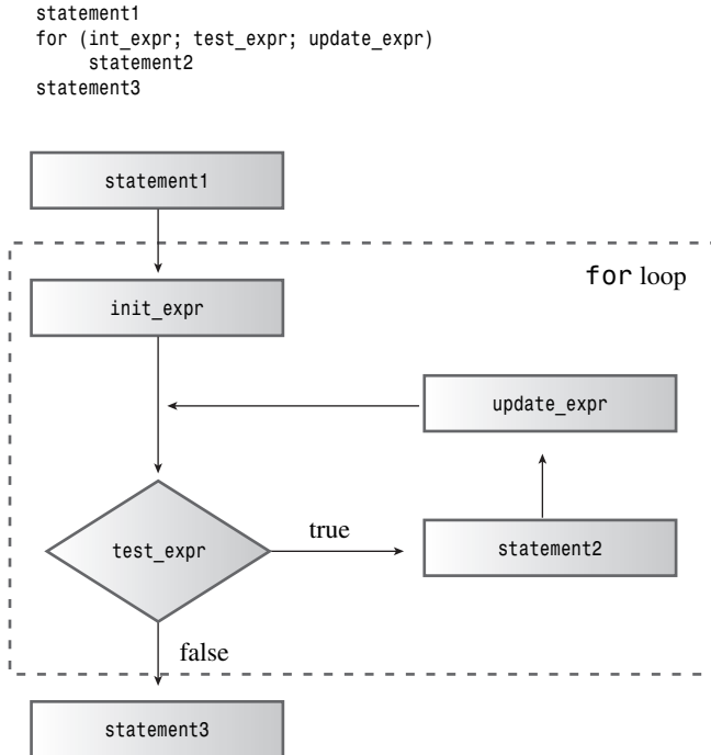
FIGURE 5.1 The design of for loops.
