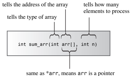
FIGURE 7.4 Telling a function about an array.
