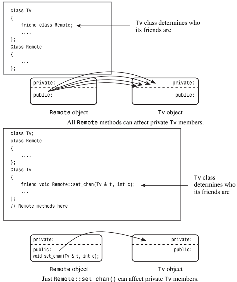
FIGURE 15.1 Class friends versus class member friends.
