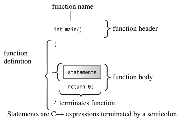
FIGURE 2.1 The main() function.
