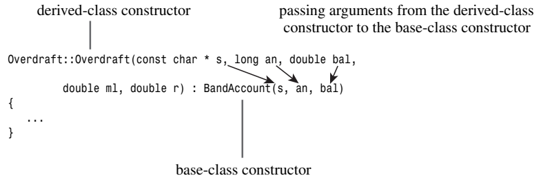
FIGURE 13.2 Passing arguments through to a base-class constructor.
