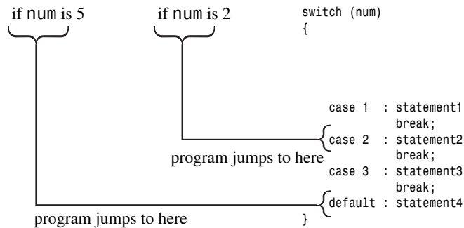
FIGURE 6.3 The structure of switch statements.
