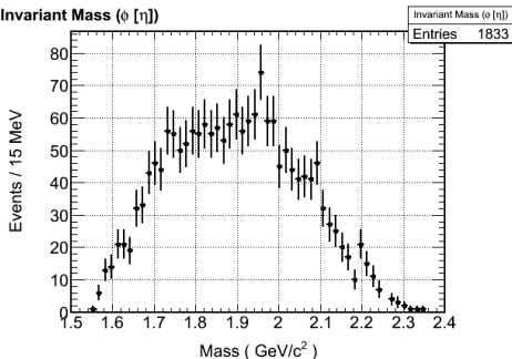
Invariant Mass ( \phi [ \eta ])
