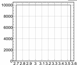
Beam3_MC_gamp_Generated
