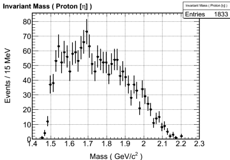
Invariant Mass ( Proton [ \eta ] )
