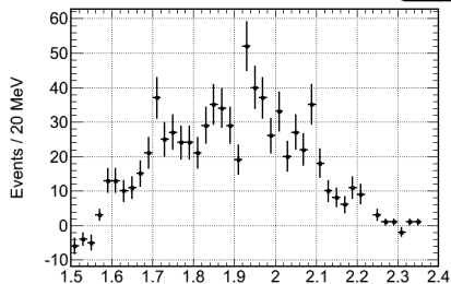
Mass_phi_eta_SideBandSubtracted
