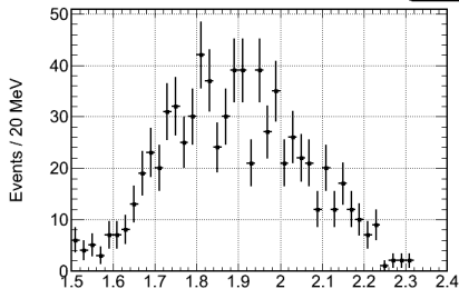
Mass_phi_eta_Left_N_Right
