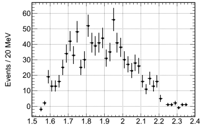
Mass_eta_phi_SideBandSubtracted
