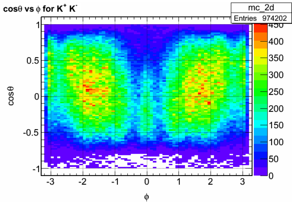
(a) MC GJ \cos\theta vs \phi
