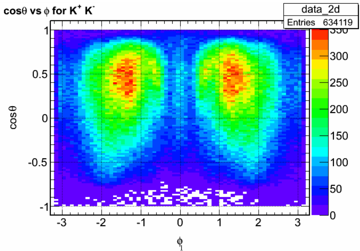
(b) Data GJ \cos\theta vs \phi
