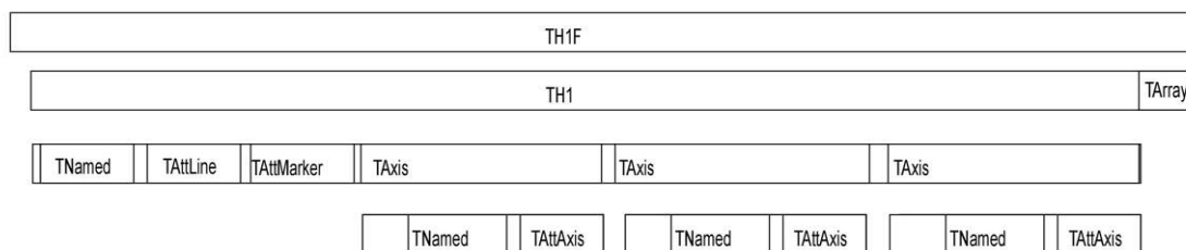
Figure 11-6 A diagram of a streamed TH1F in the buffer
