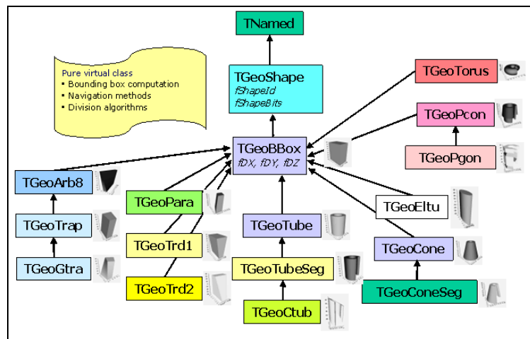
Figure 18-3 Primitive Shapes - the general inheritance scheme
