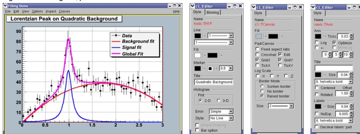
Figure 25-4 Histogram, pad and axis editors
