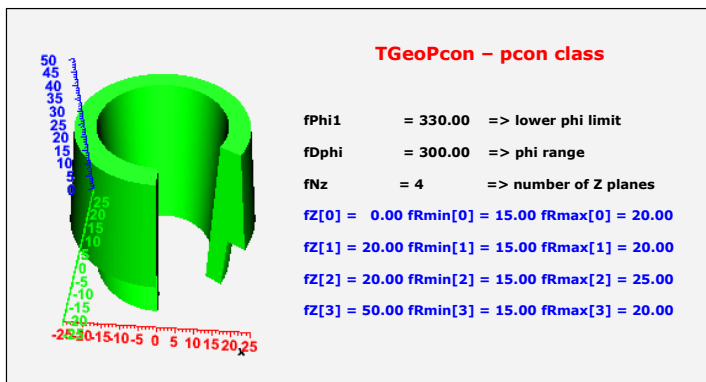
Figure 18-21 TGeoPcon Class
