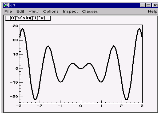
Figure 5-1 The function x \sin(x)
