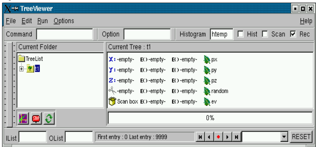
Figure 12-2 The TreeViewer
