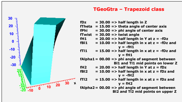
Figure 18-9 TGeoGtra class
