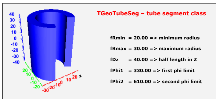
Figure 18-12 TGeoTubeSeg Class
