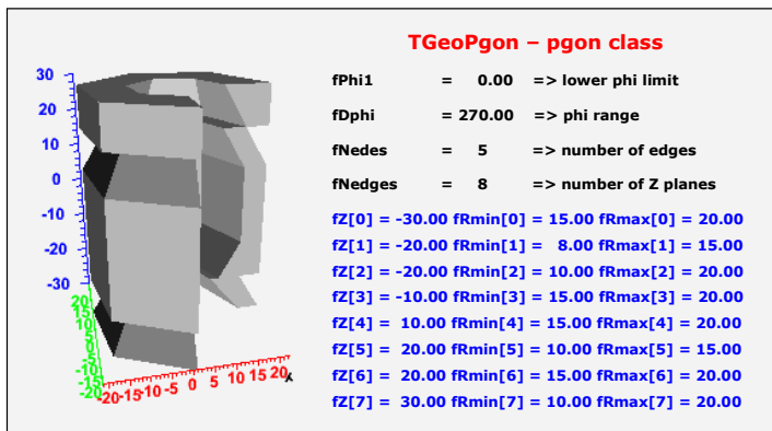
Figure 18-22 TGeoPgon Class
