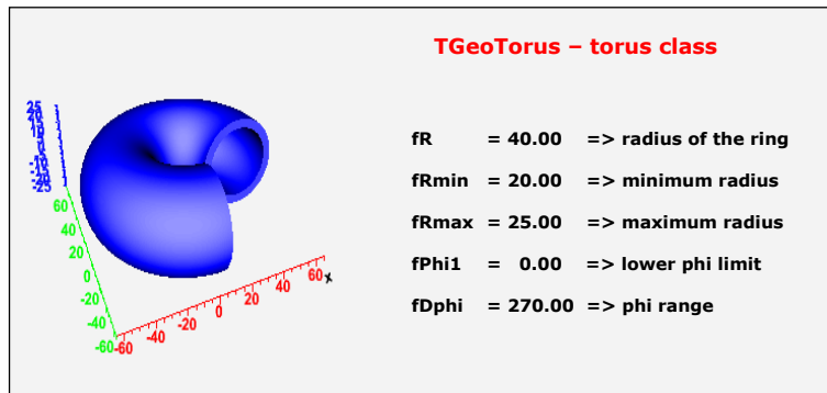
Figure 18-19 TGeoTorus Class
