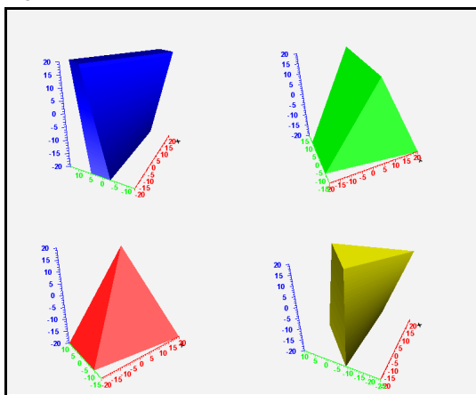
Figure 18-10 TGeoArb8 class
