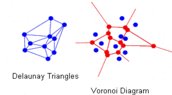
Figure 4-14 Delaunay triangles and Voronoi diagram
