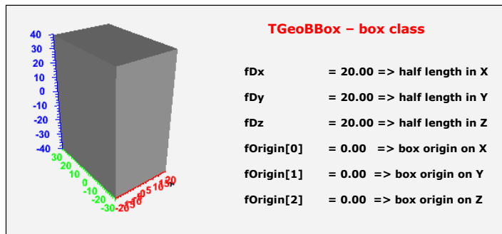
Figure 18-4 TGeoBBox class
