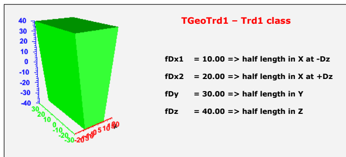
Figure 18-6 TGeoTrd1 class
