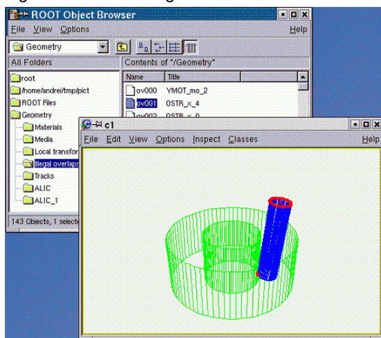
Figure 18-30 Extruding volumes
