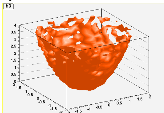
Figure 3-19 Iso surfaces
