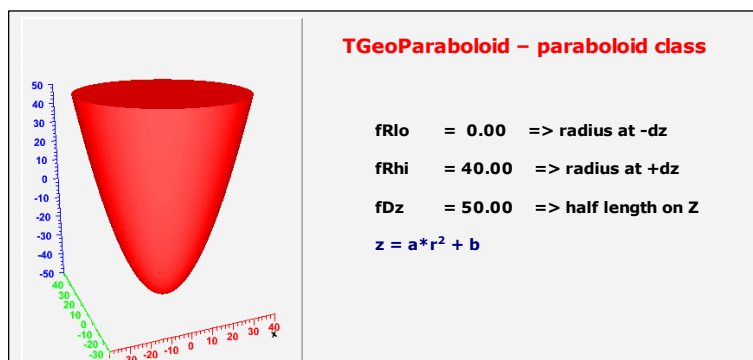
Figure 18-20 TGeoParaboloid Class
