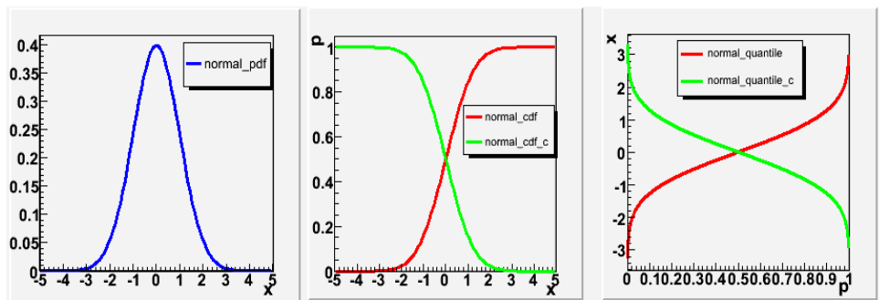
Figure 13-2 PDF, CDF and quantiles in the case of the normal distribution
