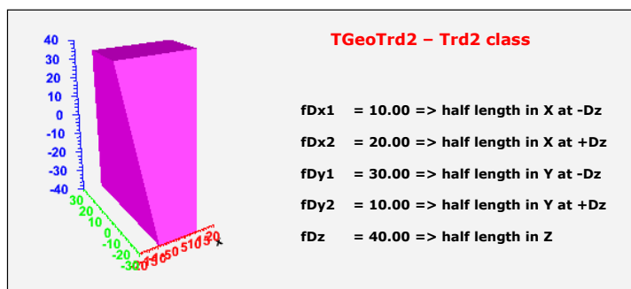
Figure 18-7 TGeoTrd2 class
