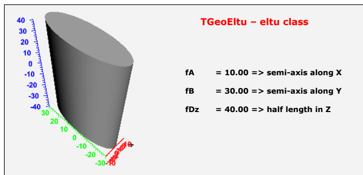
Figure 18-14 TGeoEltu Class
