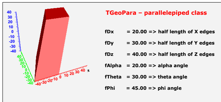
Figure 18-5 TGeoPara class
