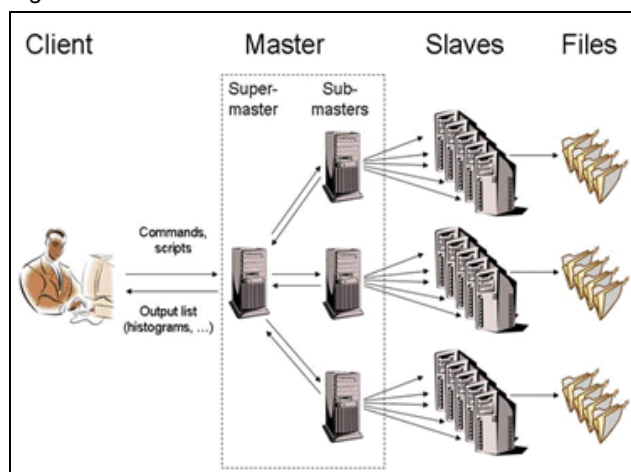
Figure 24-1 The Multi-tier structure of a PROOF cluster
