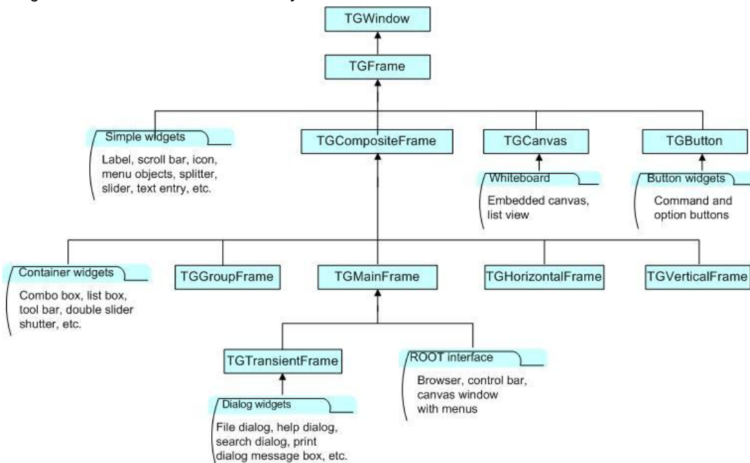
Figure 25-2 The GUI classes hierarchy
