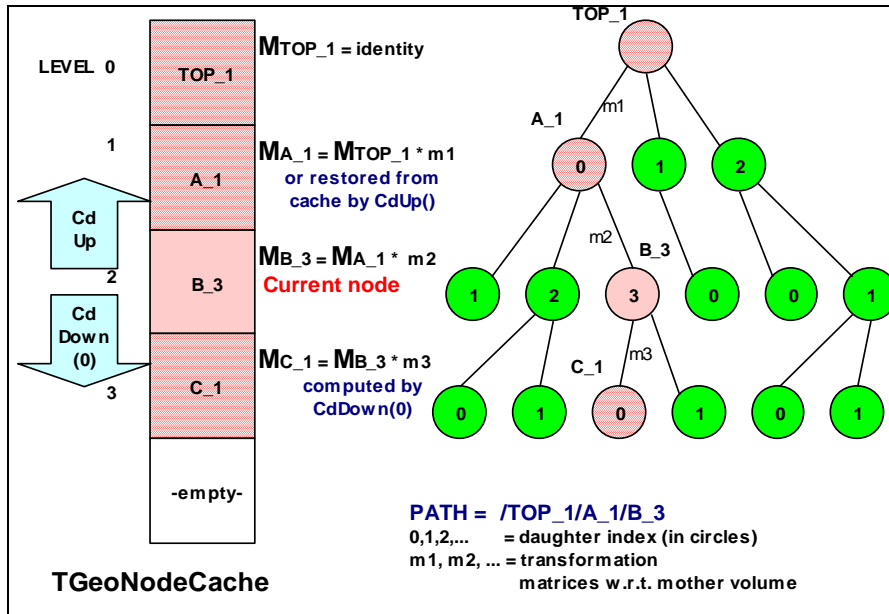
Figure 18-37 Navigation in the geometry hierarchy
