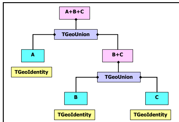
Figure 18-25 Representation of A+B+C
