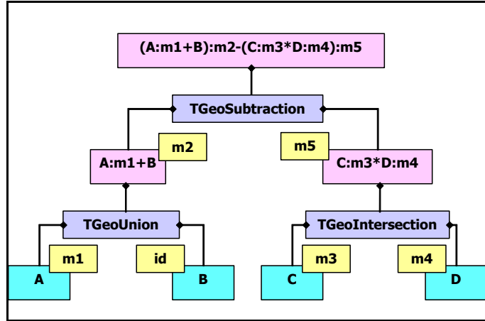
Figure 18-26 Internal representation for composite shapes
