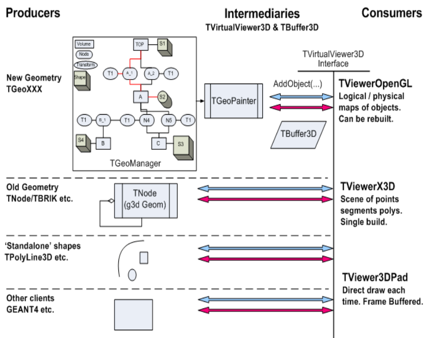
Figure 9-36 Overview of 3D viewer architecture
