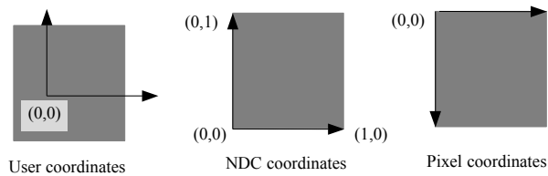
Figure 9-3 Pad coordinate systems
