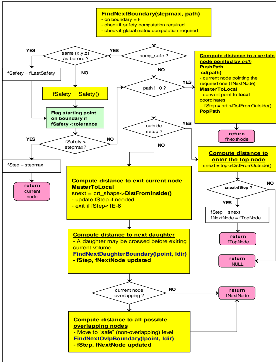
Figure 18-39 Finding the distance to the next crossed boundary
