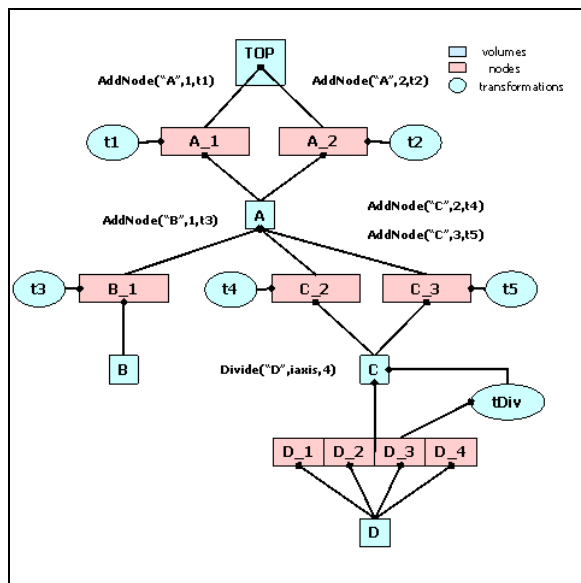
Figure 18-28 A geometry hierarchy in memory
