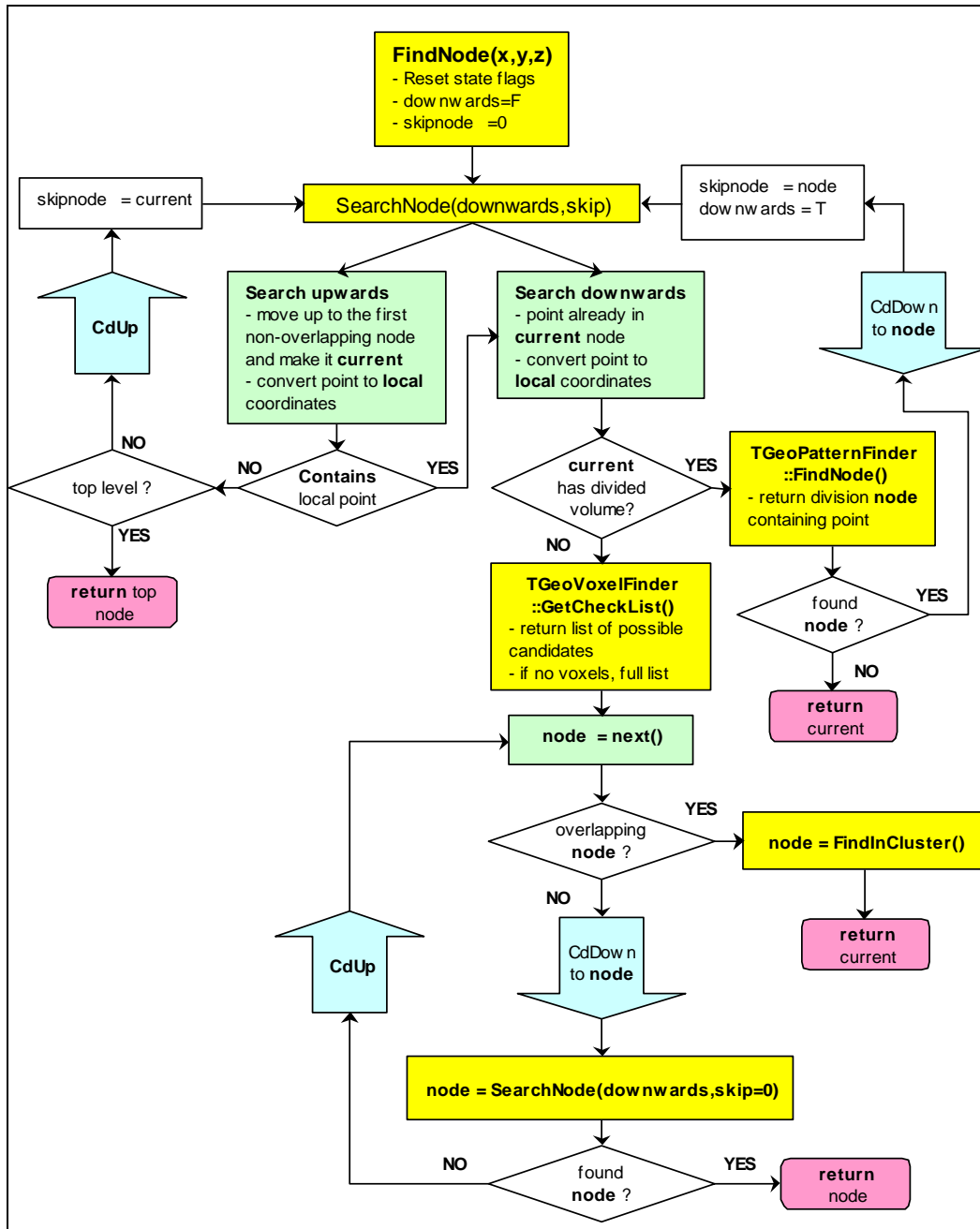
Figure 18-38 Finding the location of a point in the geometry hierarchy
