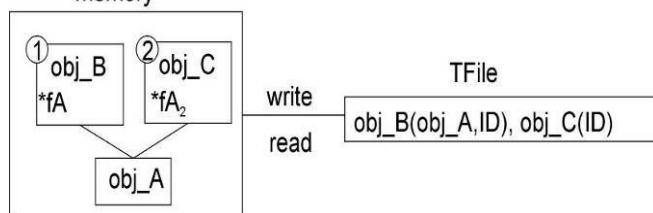
Figure 11-7 Streaming object pointers memory
