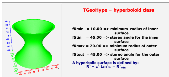
Figure 18-15 TGeoHype Class
