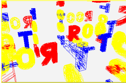
Figure 18-34 Random rays
