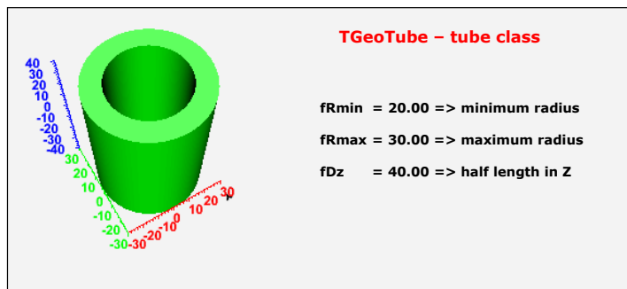
Figure 18-11 TGeoTube Class
