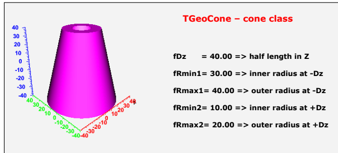
Figure 18-16 TGeoCone Class
