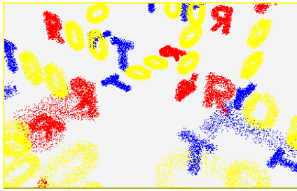
Figure 18-33 Random points
