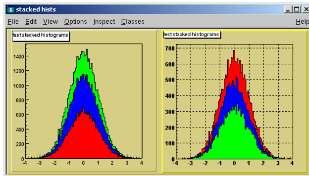
Figure 3-16 Stacked histograms
