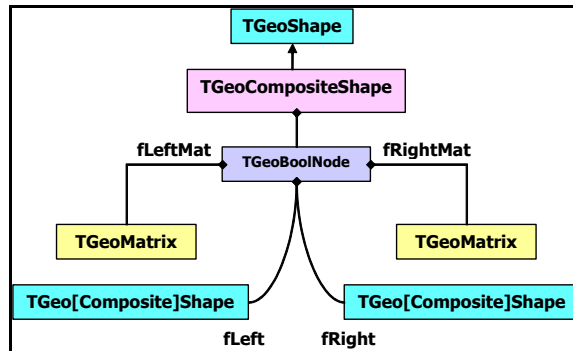
Figure 18-24 The composite shapes structure
