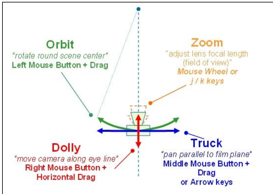
Figure 9-32 GL Viewer camera interactions
